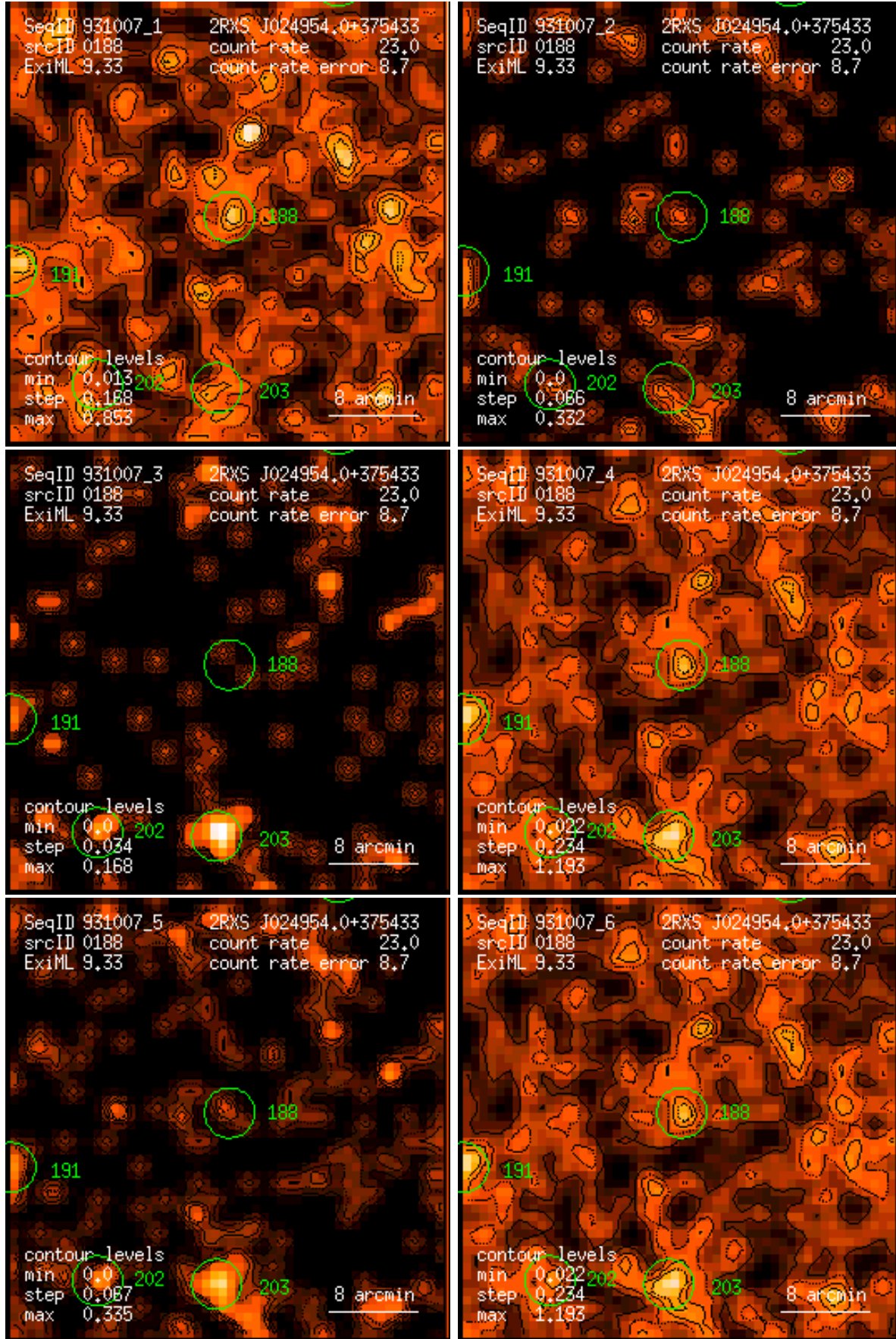
Figure 188: RASS 931007: detection 0188: band rate images, Gaussian filter: (1) PSPC channels 11 – 41, (2) 52 – 90, (3) 91 – 201, (4) 11 – 235, (5) 52 – 201, (6) 11 – 201. Broad band rates in counts/ks. Band rate contour levels in counts/ks/arcmin 2 .
