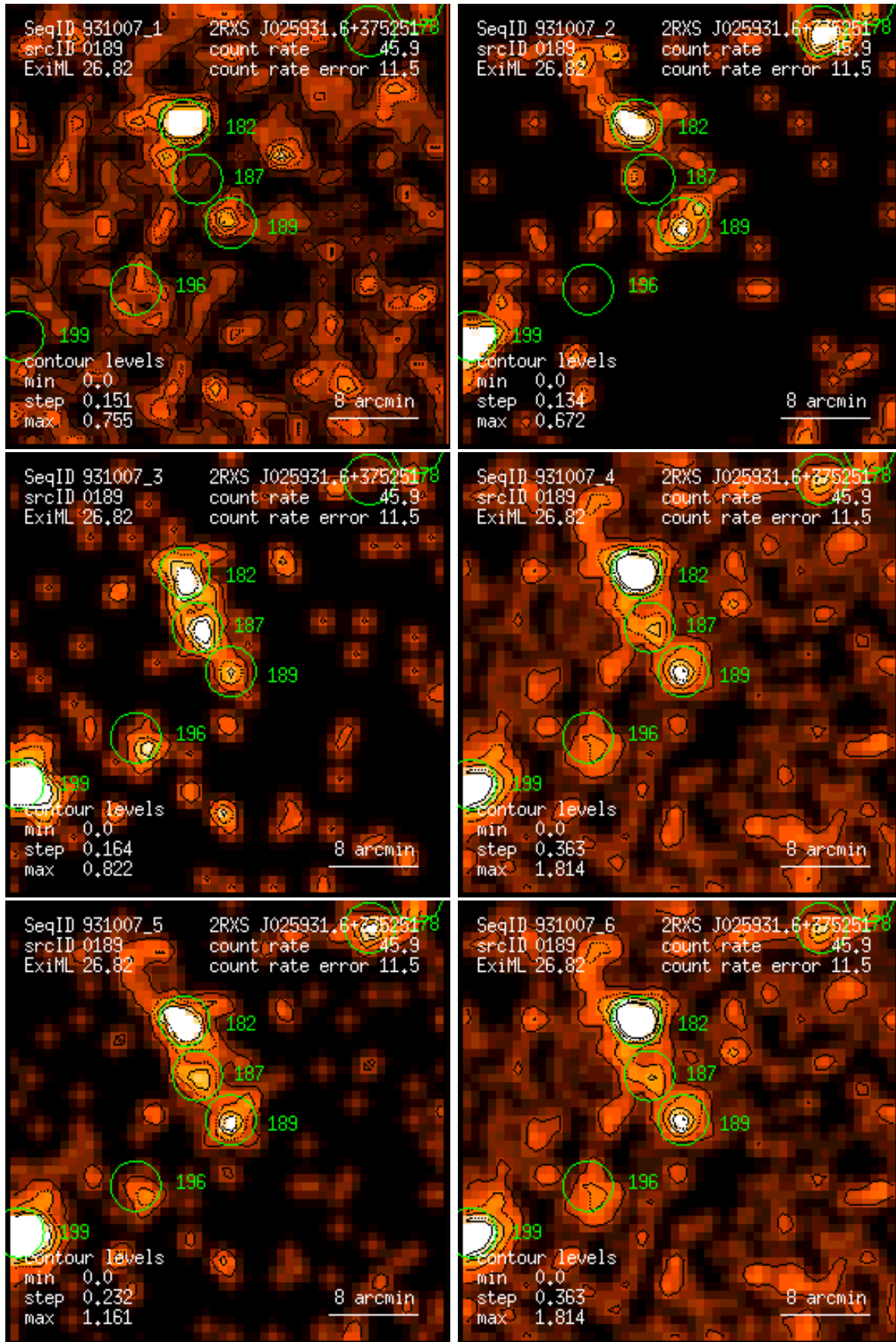
Figure 189: RASS 931007: detection 0189: band rate images, Gaussian filter: (1) PSPC channels 11 – 41, (2) 52 – 90, (3) 91 – 201, (4) 11 – 235, (5) 52 – 201, (6) 11 – 201. Broad band rates in counts/ks. Band rate contour levels in counts/ks/arcmin 2 .
