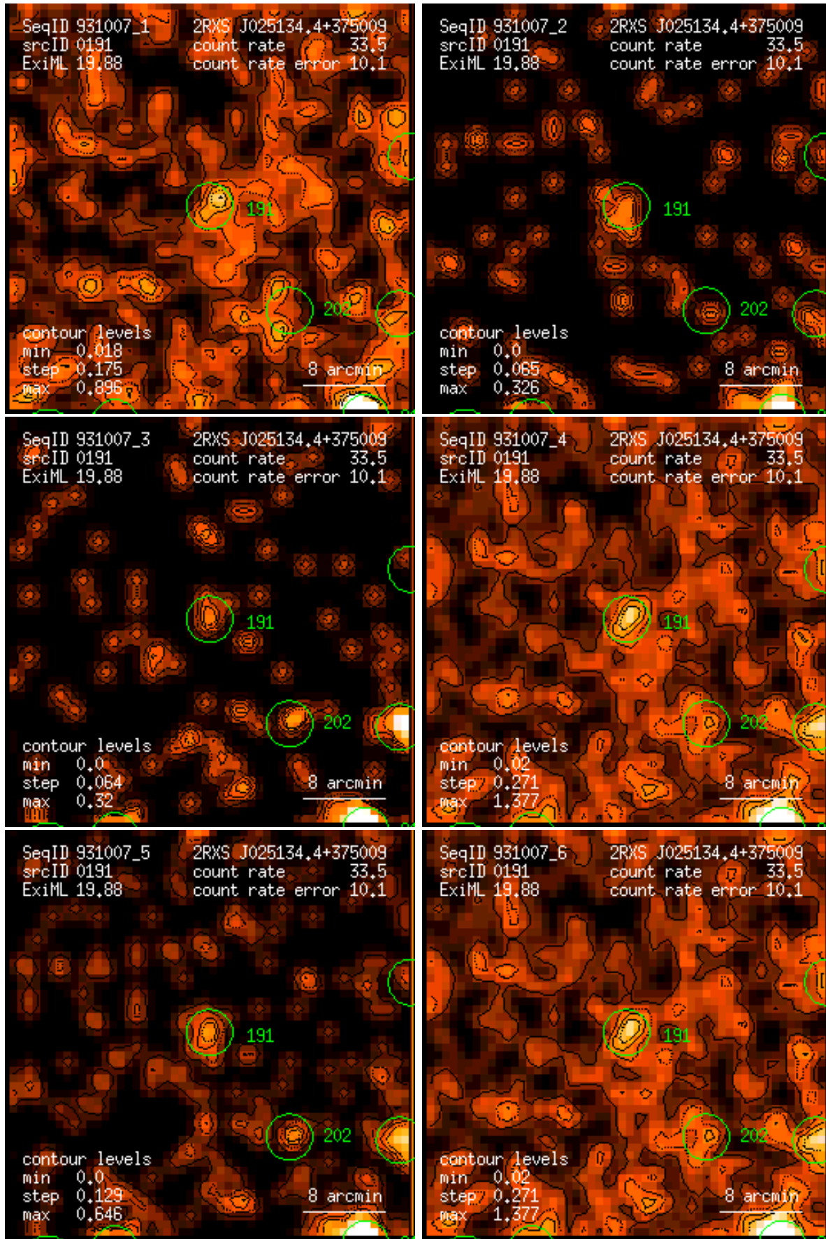
Figure 191: RASS 931007: detection 0191: band rate images, Gaussian filter: (1) PSPC channels 11 – 41, (2) 52 – 90, (3) 91 – 201, (4) 11 – 235, (5) 52 – 201, (6) 11 – 201. Broad band rates in counts/ks. Band rate contour levels in counts/ks/arcmin 2 .
