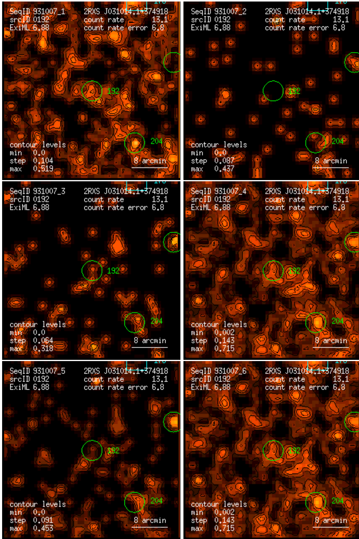
Figure 192: RASS 931007: detection 0192: band rate images, Gaussian filter: (1) PSPC channels 11 – 41, (2) 52 – 90, (3) 91 – 201, (4) 11 – 235, (5) 52 – 201, (6) 11 – 201. Broad band rates in counts/ks. Band rate contour levels in counts/ks/arcmin 2 .
