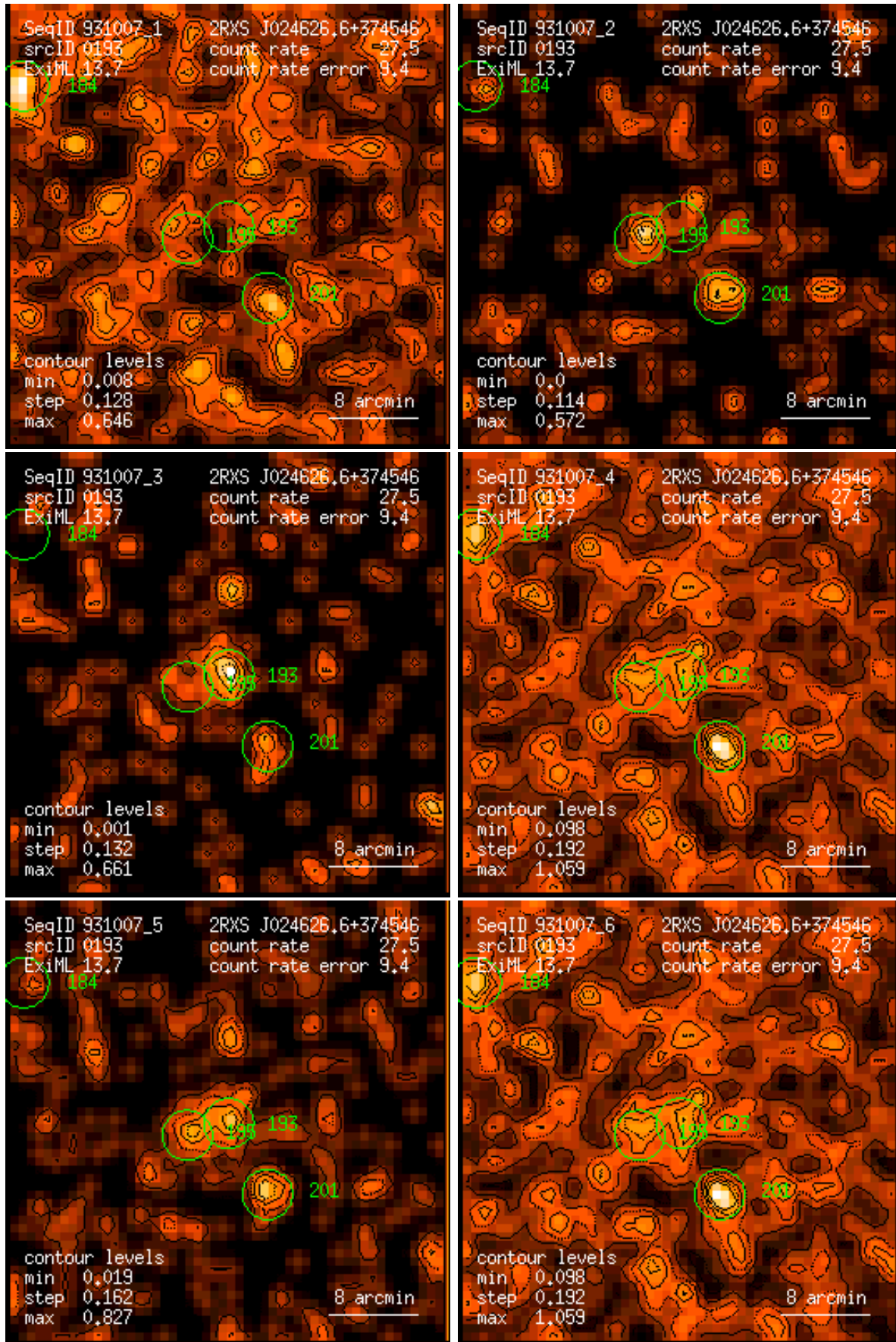
Figure 193: RASS 931007: detection 0193: band rate images, Gaussian filter: (1) PSPC channels 11 – 41, (2) 52 – 90, (3) 91 – 201, (4) 11 – 235, (5) 52 – 201, (6) 11 – 201. Broad band rates in counts/ks. Band rate contour levels in counts/ks/arcmin 2 .
