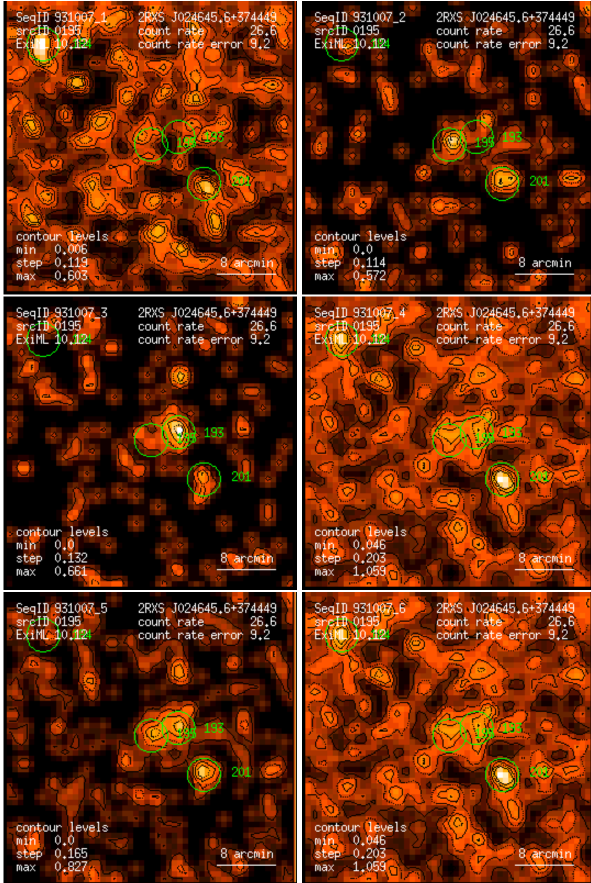
Figure 195: RASS 931007: detection 0195: band rate images, Gaussian filter: (1) PSPC channels 11 – 41, (2) 52 – 90, (3) 91 – 201, (4) 11 – 235, (5) 52 – 201, (6) 11 – 201. Broad band rates in counts/ks. Band rate contour levels in counts/ks/arcmin 2 .
