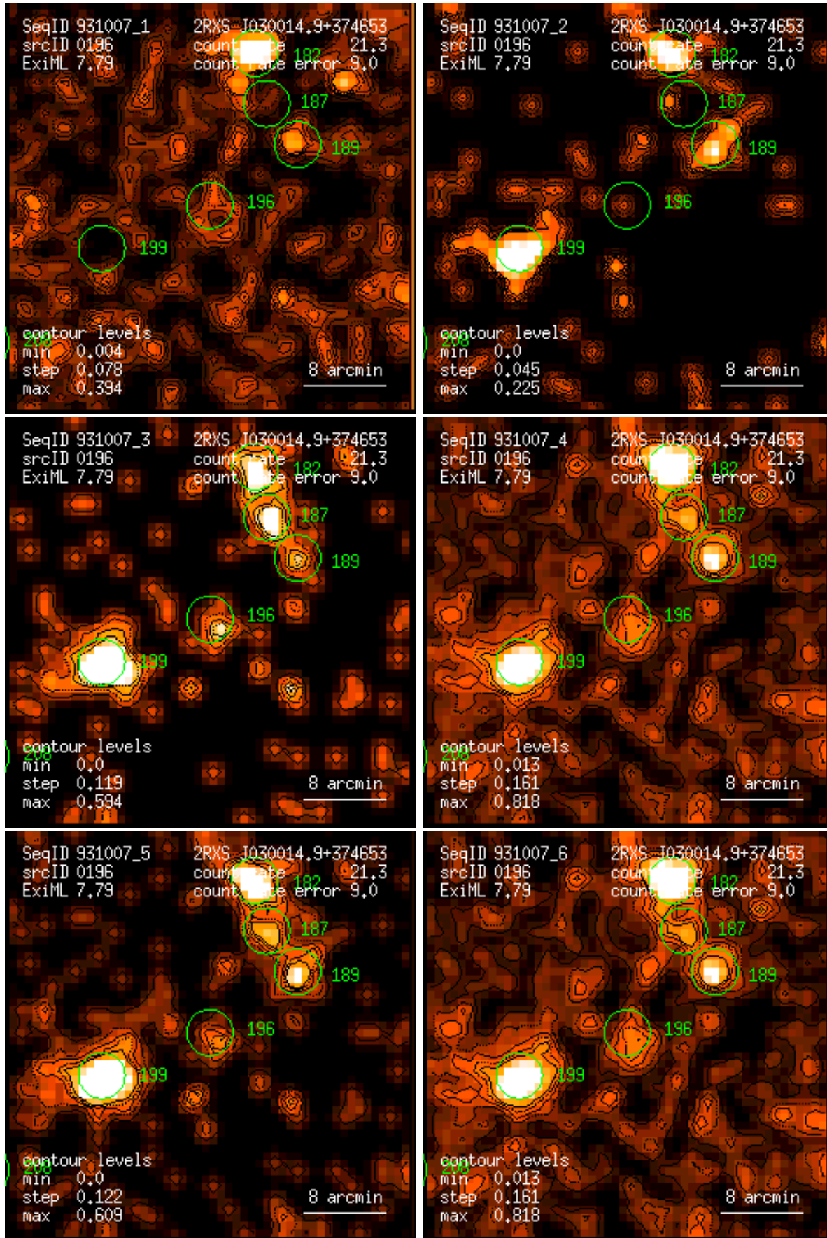
Figure 196: RASS 931007: detection 0196: band rate images, Gaussian filter: (1) PSPC channels 11 – 41, (2) 52 – 90, (3) 91 – 201, (4) 11 – 235, (5) 52 – 201, (6) 11 – 201. Broad band rates in counts/ks. Band rate contour levels in counts/ks/arcmin 2 .
