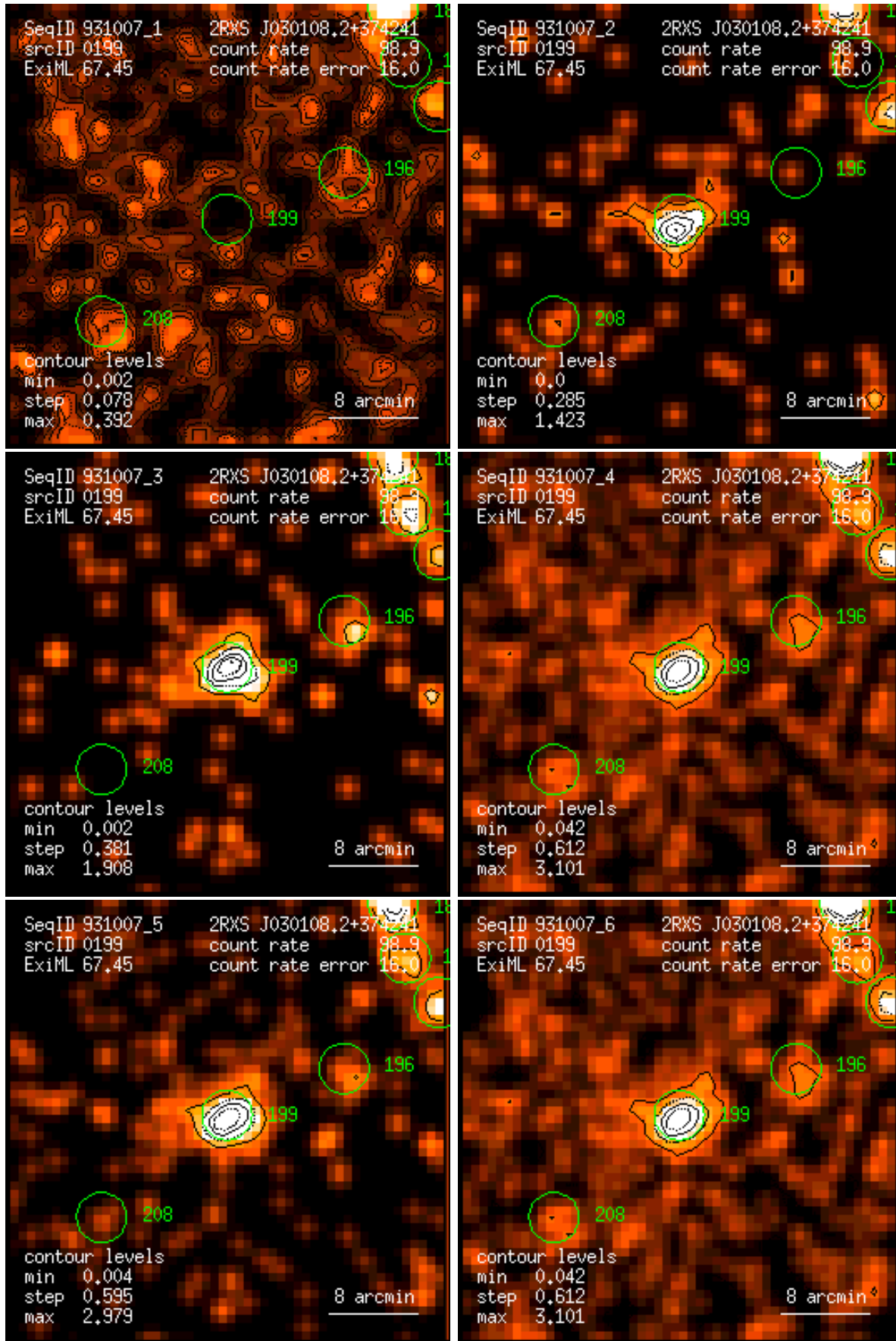
Figure 199: RASS 931007: detection 0199: band rate images, Gaussian filter: (1) PSPC channels 11 – 41, (2) 52 – 90, (3) 91 – 201, (4) 11 – 235, (5) 52 – 201, (6) 11 – 201. Broad band rates in counts/ks. Band rate contour levels in counts/ks/arcmin 2 .
