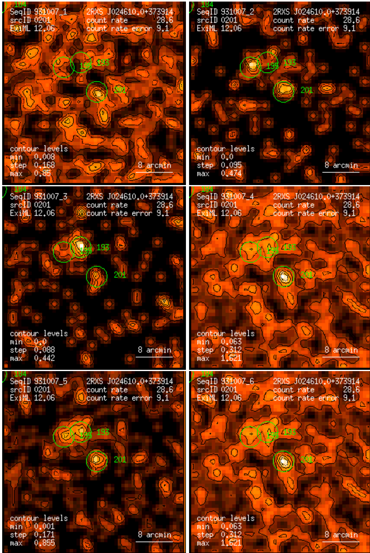
Figure 201: RASS 931007: detection 0201: band rate images, Gaussian filter: (1) PSPC channels 11 – 41, (2) 52 – 90, (3) 91 – 201, (4) 11 – 235, (5) 52 – 201, (6) 11 – 201. Broad band rates in counts/ks. Band rate contour levels in counts/ks/arcmin 2 .
