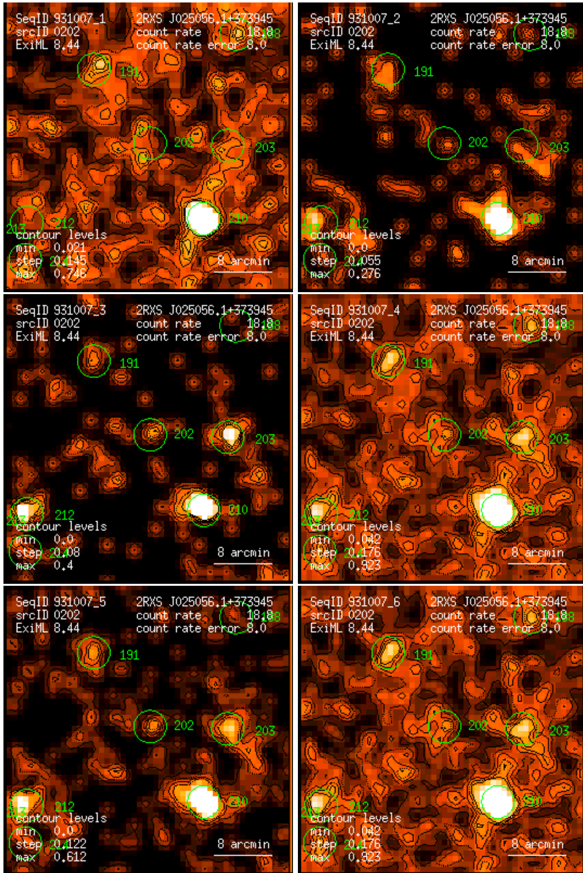
Figure 202: RASS 931007: detection 0202: band rate images, Gaussian filter: (1) PSPC channels 11 – 41, (2) 52 – 90, (3) 91 – 201, (4) 11 – 235, (5) 52 – 201, (6) 11 – 201. Broad band rates in counts/ks. Band rate contour levels in counts/ks/arcmin 2 .
