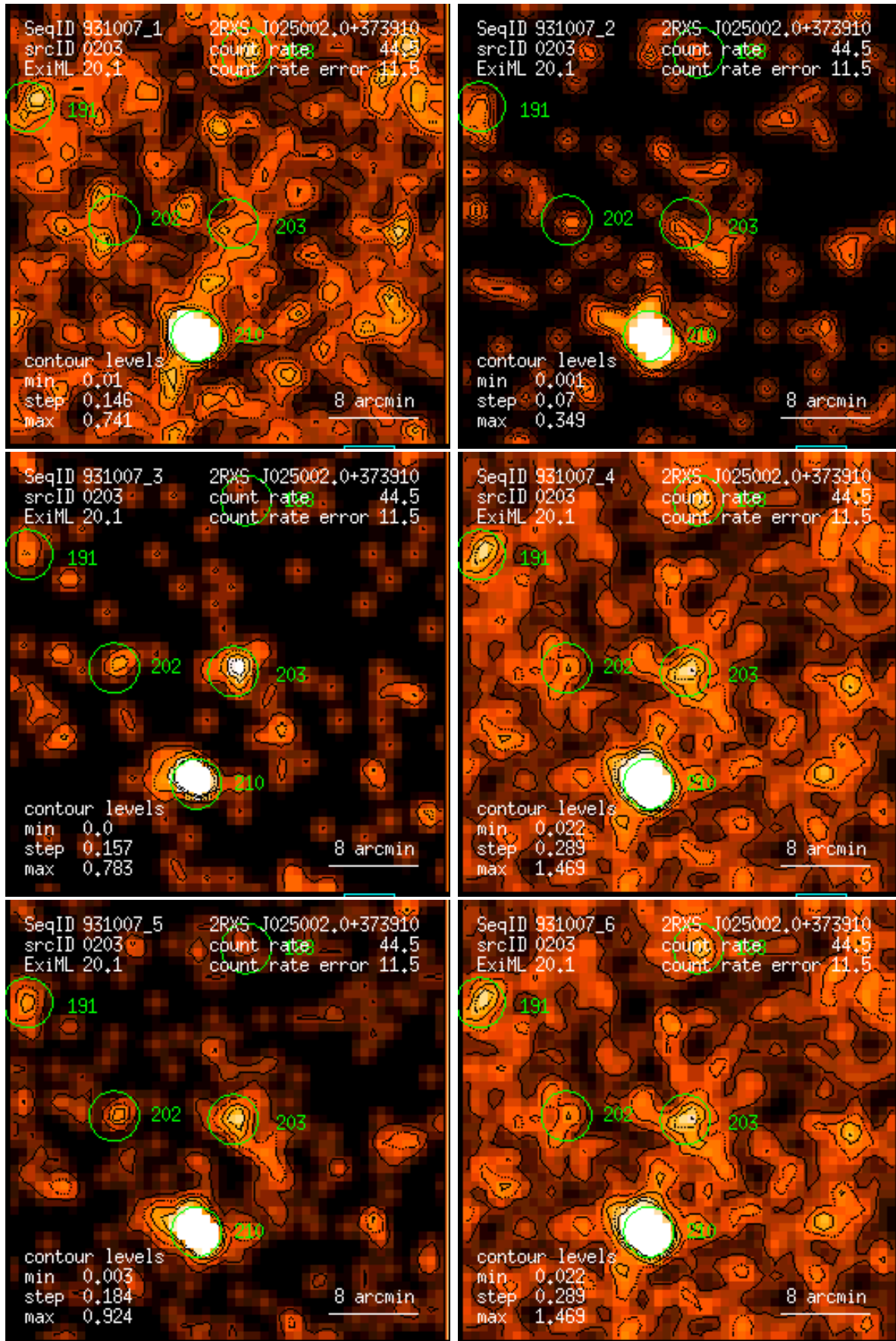
Figure 203: RASS 931007: detection 0203: band rate images, Gaussian filter: (1) PSPC channels 11 – 41, (2) 52 – 90, (3) 91 – 201, (4) 11 – 235, (5) 52 – 201, (6) 11 – 201. Broad band rates in counts/ks. Band rate contour levels in counts/ks/arcmin 2 .
