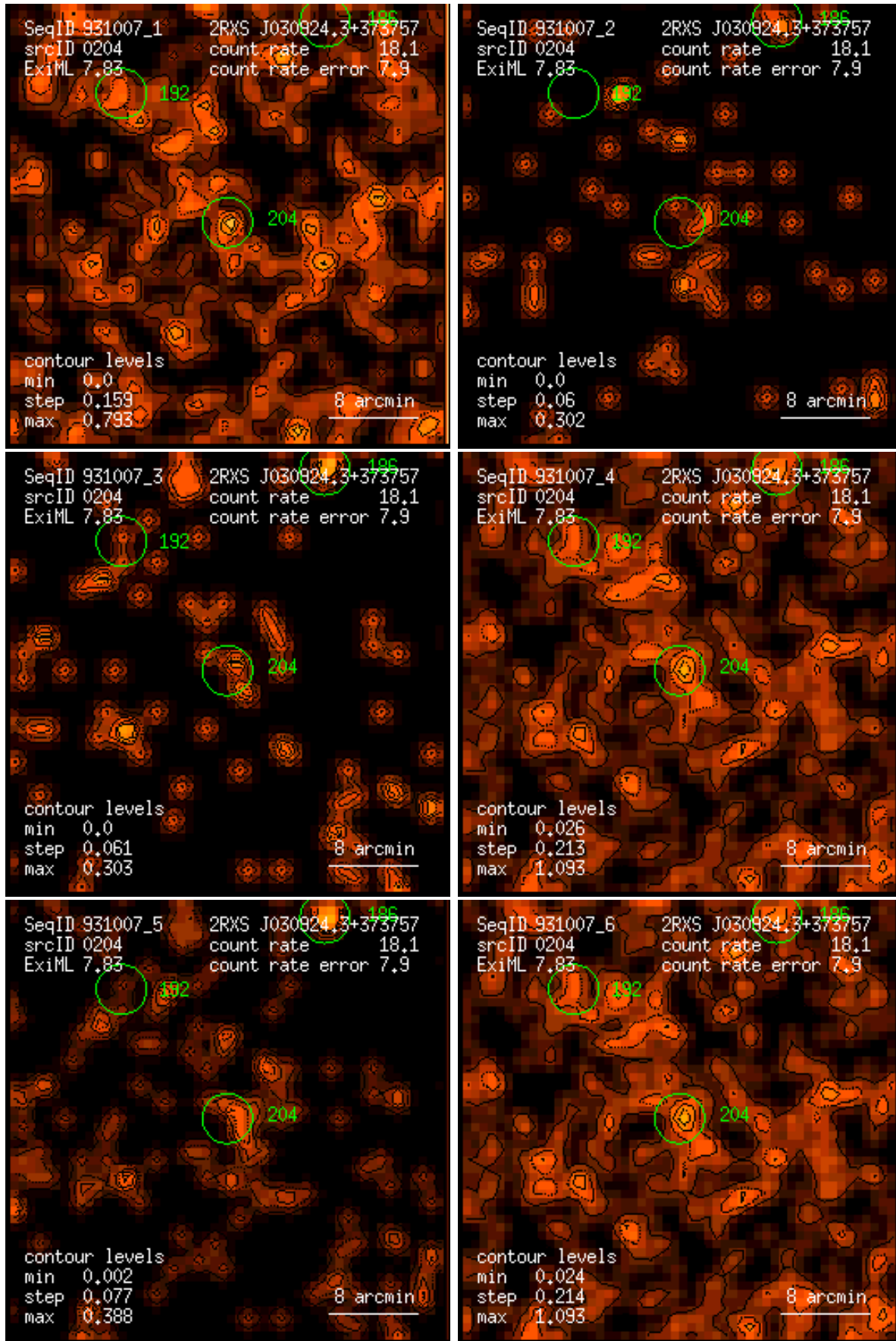
Figure 204: RASS 931007: detection 0204: band rate images, Gaussian filter: (1) PSPC channels 11 – 41, (2) 52 – 90, (3) 91 – 201, (4) 11 – 235, (5) 52 – 201, (6) 11 – 201. Broad band rates in counts/ks. Band rate contour levels in counts/ks/arcmin 2 .
