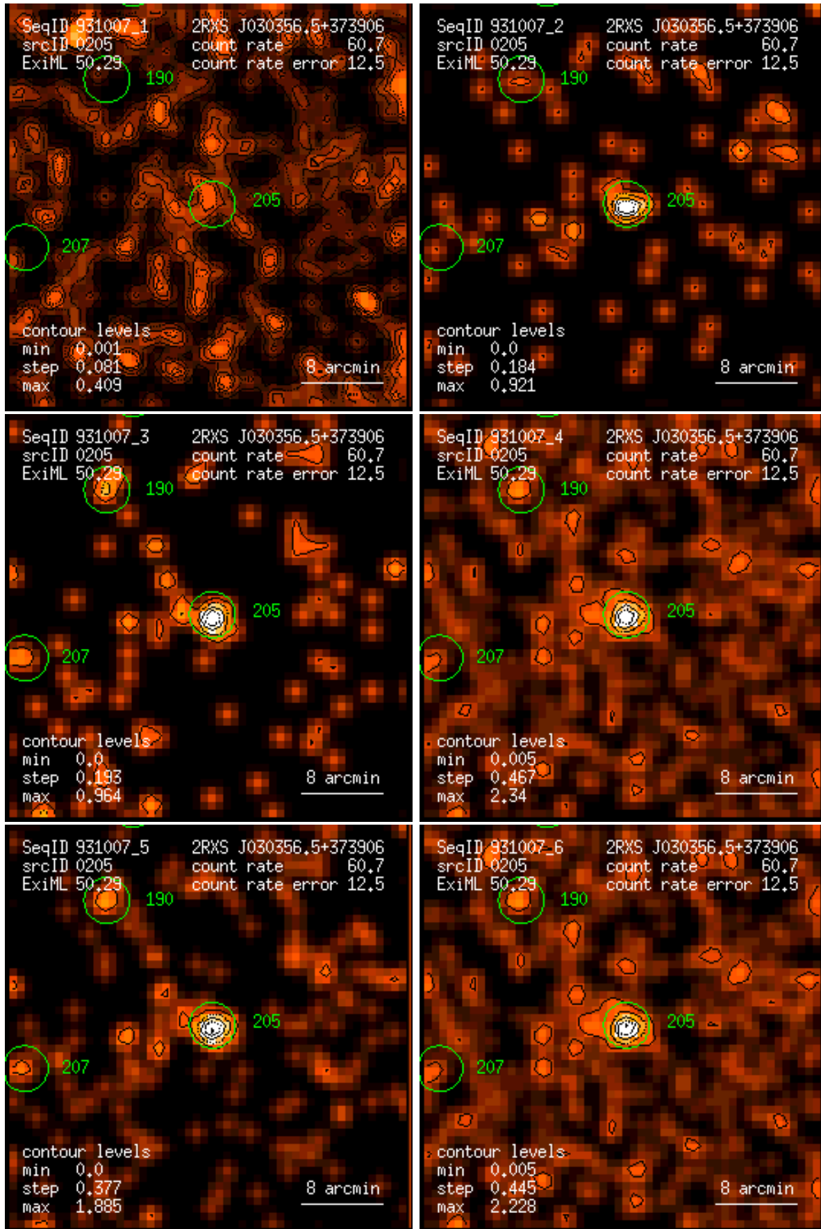
Figure 205: RASS 931007: detection 0205: band rate images, Gaussian filter: (1) PSPC channels 11 – 41, (2) 52 – 90, (3) 91 – 201, (4) 11 – 235, (5) 52 – 201, (6) 11 – 201. Broad band rates in counts/ks. Band rate contour levels in counts/ks/arcmin 2 .
