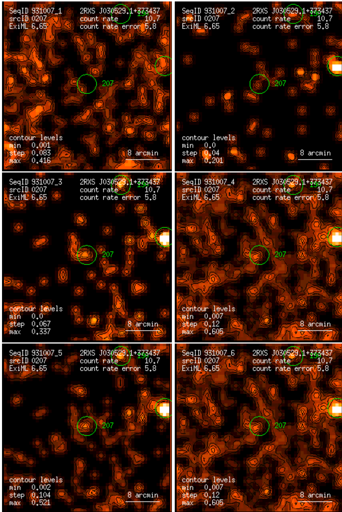
Figure 207: RASS 931007: detection 0207: band rate images, Gaussian filter: (1) PSPC channels 11 – 41, (2) 52 – 90, (3) 91 – 201, (4) 11 – 235, (5) 52 – 201, (6) 11 – 201. Broad band rates in counts/ks. Band rate contour levels in counts/ks/arcmin 2 .
