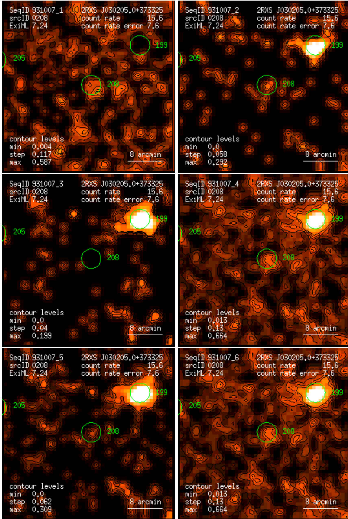
Figure 208: RASS 931007: detection 0208: band rate images, Gaussian filter: (1) PSPC channels 11 – 41, (2) 52 – 90, (3) 91 – 201, (4) 11 – 235, (5) 52 – 201, (6) 11 – 201. Broad band rates in counts/ks. Band rate contour levels in counts/ks/arcmin 2 .
