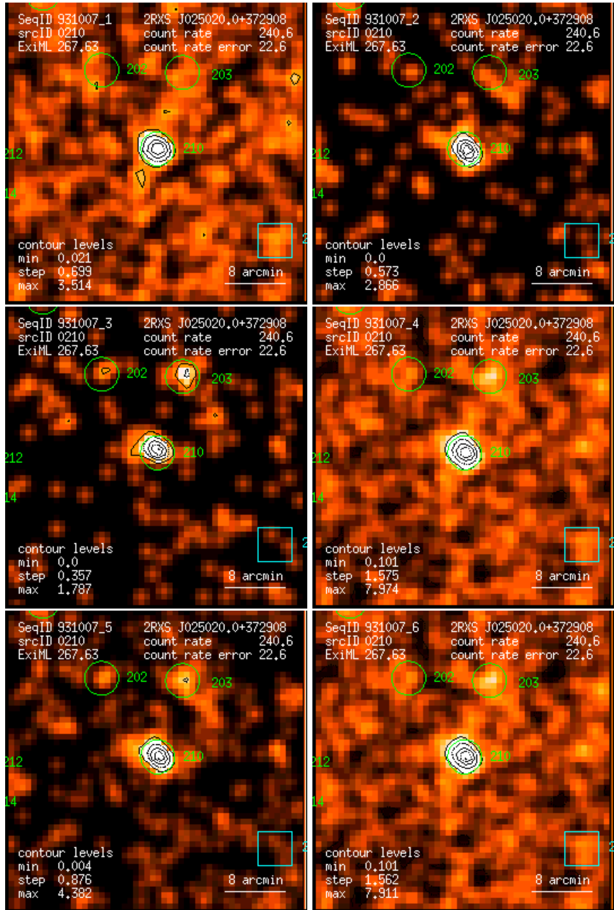
Figure 210: RASS 931007: detection 0210: band rate images, Gaussian filter: (1) PSPC channels 11 – 41, (2) 52 – 90, (3) 91 – 201, (4) 11 – 235, (5) 52 – 201, (6) 11 – 201. Broad band rates in counts/ks. Band rate contour levels in counts/ks/arcmin 2 .
