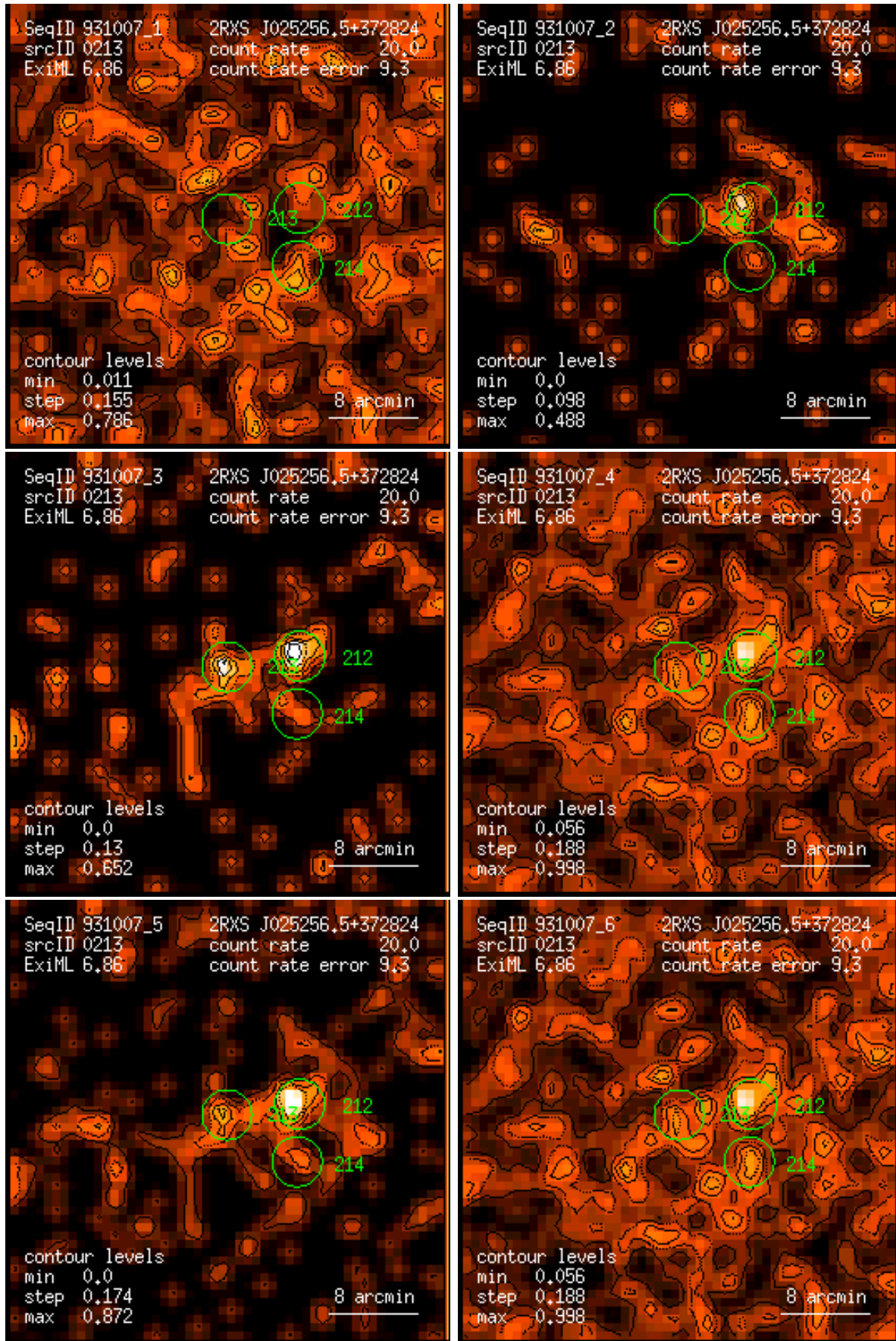
Figure 213: RASS 931007: detection 0213: band rate images, Gaussian filter: (1) PSPC channels 11 – 41, (2) 52 – 90, (3) 91 – 201, (4) 11 – 235, (5) 52 – 201, (6) 11 – 201. Broad band rates in counts/ks. Band rate contour levels in counts/ks/arcmin 2 .
