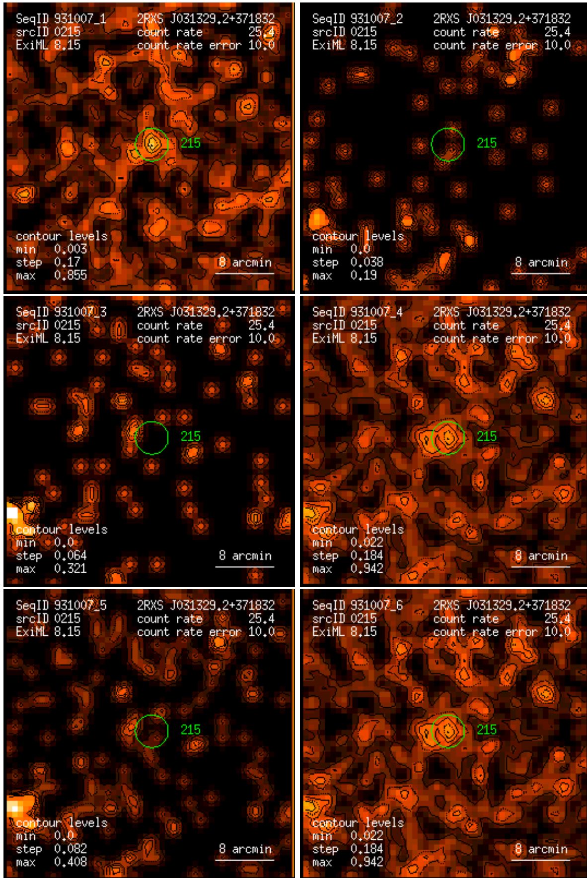
Figure 215: RASS 931007: detection 0215: band rate images, Gaussian filter: (1) PSPC channels 11 – 41, (2) 52 – 90, (3) 91 – 201, (4) 11 – 235, (5) 52 – 201, (6) 11 – 201. Broad band rates in counts/ks. Band rate contour levels in counts/ks/arcmin 2 .
