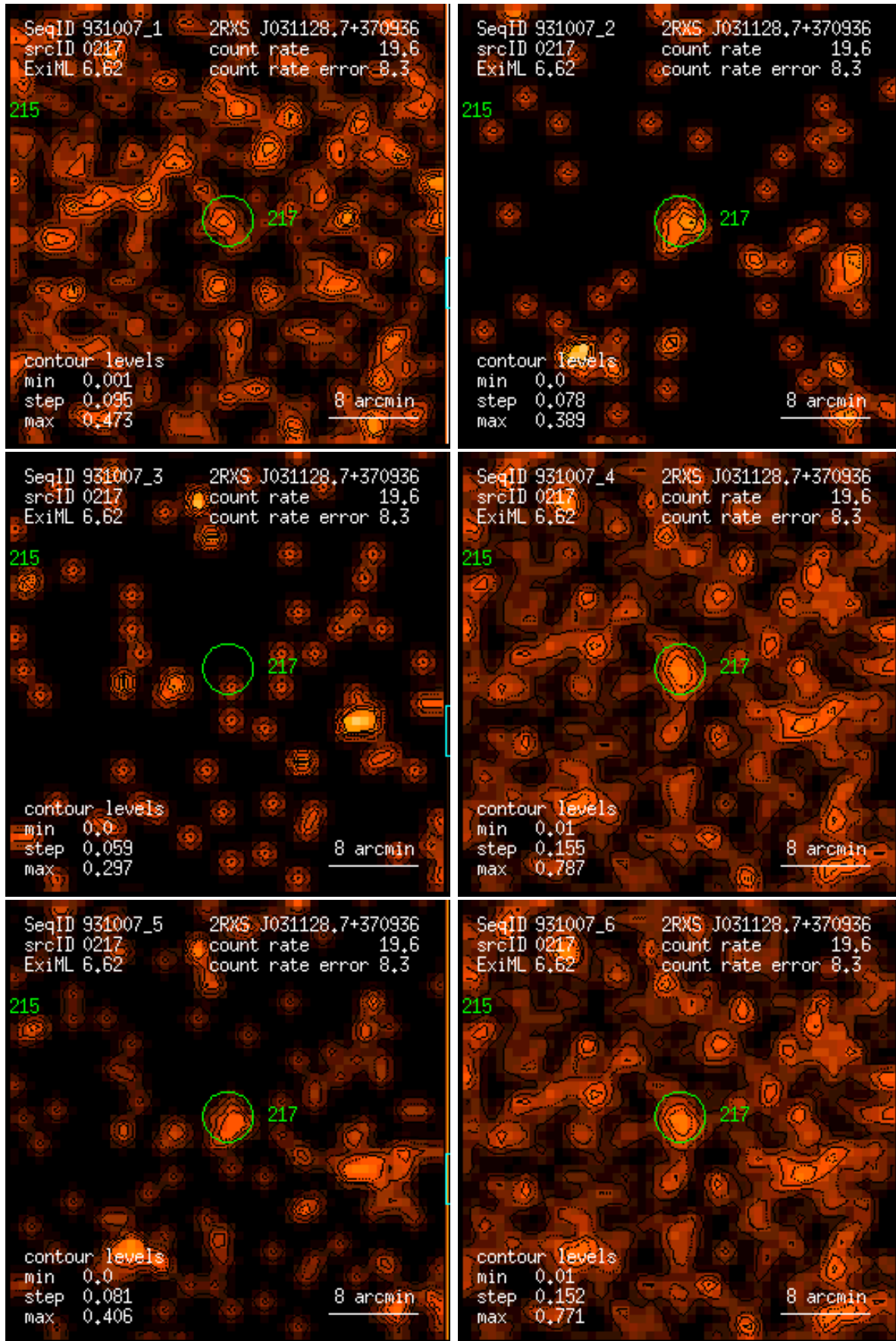
Figure 217: RASS 931007: detection 0217: band rate images, Gaussian filter: (1) PSPC channels 11 – 41, (2) 52 – 90, (3) 91 – 201, (4) 11 – 235, (5) 52 – 201, (6) 11 – 201. Broad band rates in counts/ks. Band rate contour levels in counts/ks/arcmin 2 .
