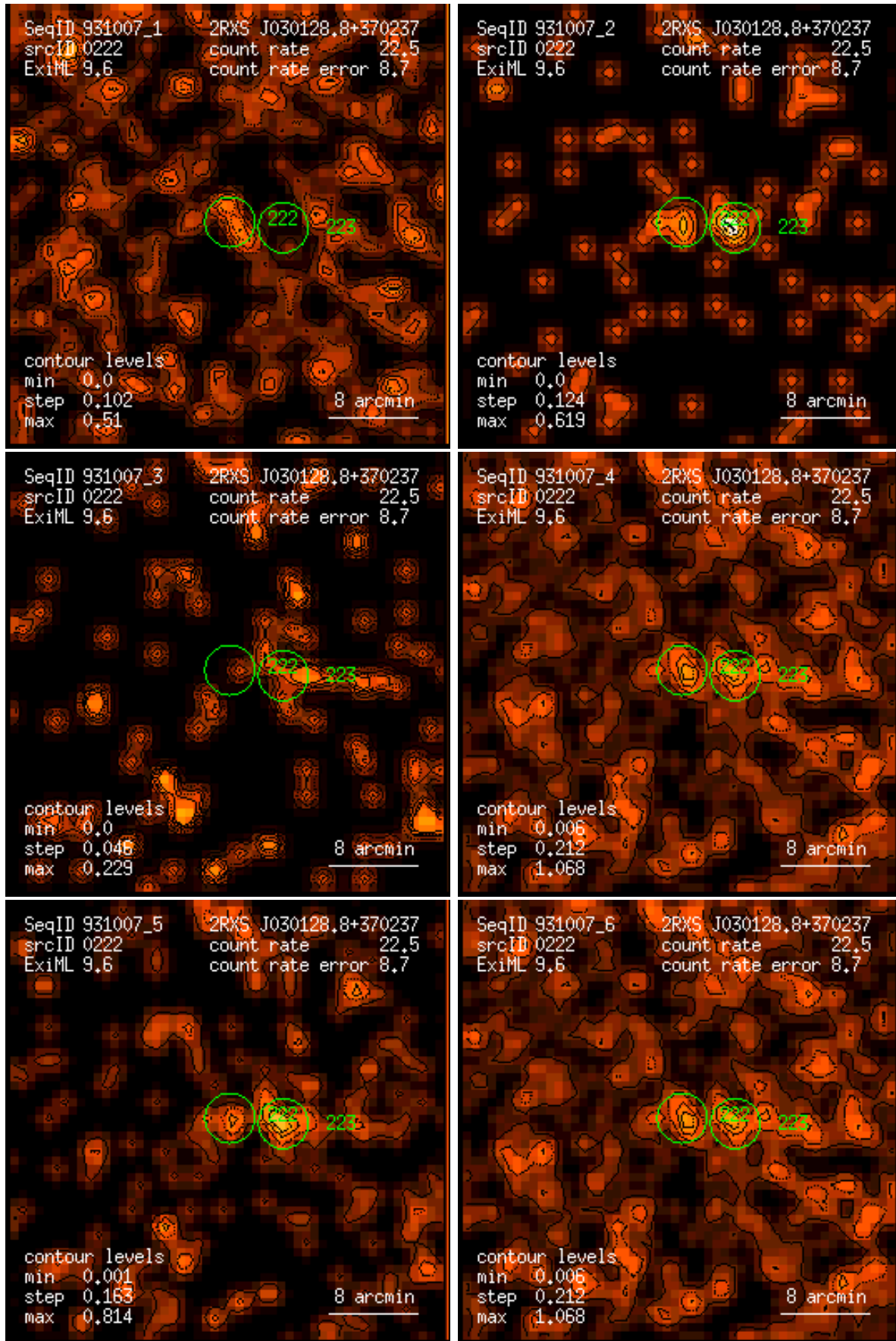
Figure 222: RASS 931007: detection 0222: band rate images, Gaussian filter: (1) PSPC channels 11 – 41, (2) 52 – 90, (3) 91 – 201, (4) 11 – 235, (5) 52 – 201, (6) 11 – 201. Broad band rates in counts/ks. Band rate contour levels in counts/ks/arcmin 2 .
