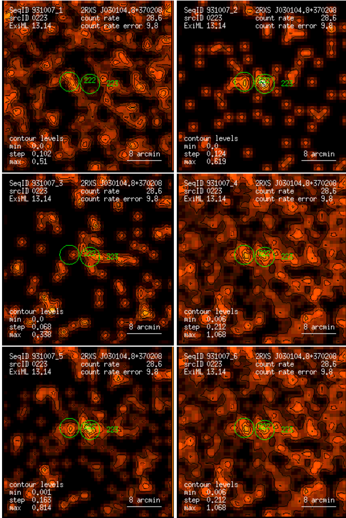
Figure 223: RASS 931007: detection 0223: band rate images, Gaussian filter: (1) PSPC channels 11 – 41, (2) 52 – 90, (3) 91 – 201, (4) 11 – 235, (5) 52 – 201, (6) 11 – 201. Broad band rates in counts/ks. Band rate contour levels in counts/ks/arcmin 2 .
