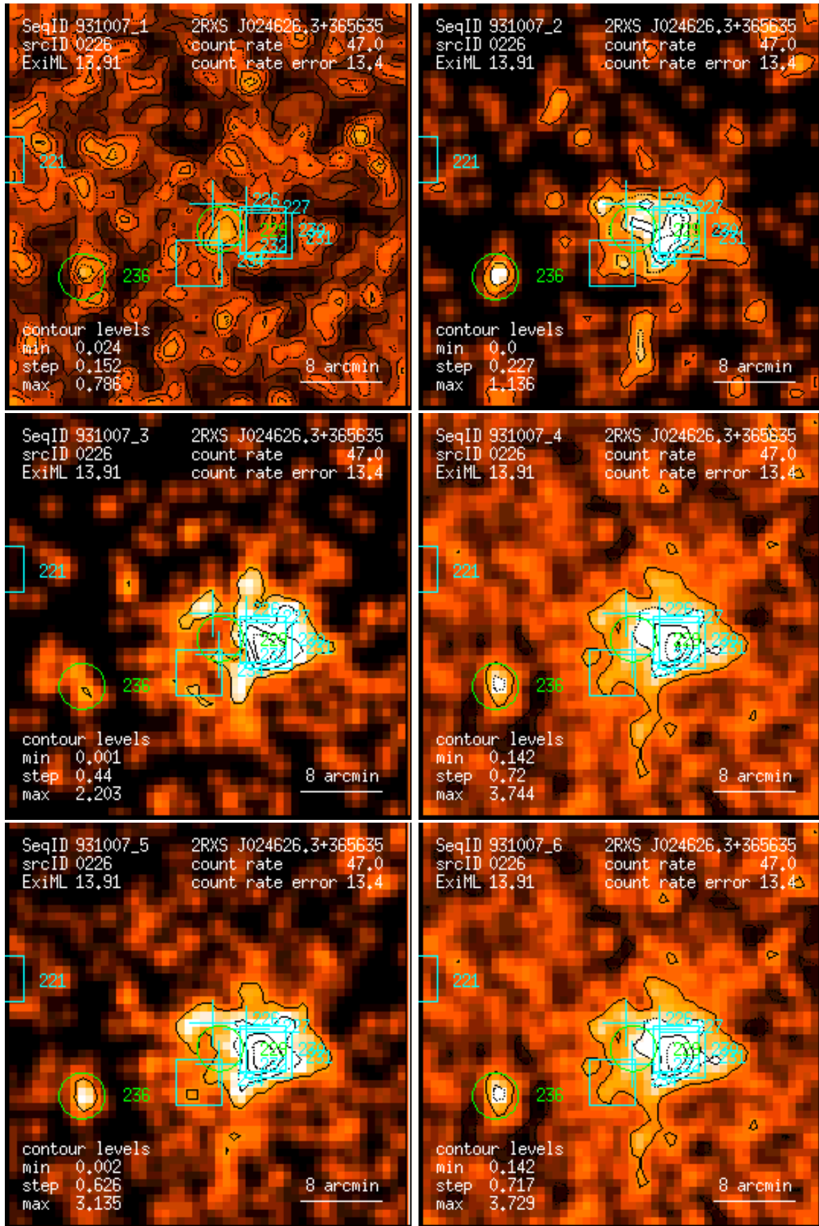
Figure 226: RASS 931007: detection 0226: band rate images, Gaussian filter: (1) PSPC channels 11 – 41, (2) 52 – 90, (3) 91 – 201, (4) 11 – 235, (5) 52 – 201, (6) 11 – 201. Broad band rates in counts/ks. Band rate contour levels in counts/ks/arcmin 2 .
