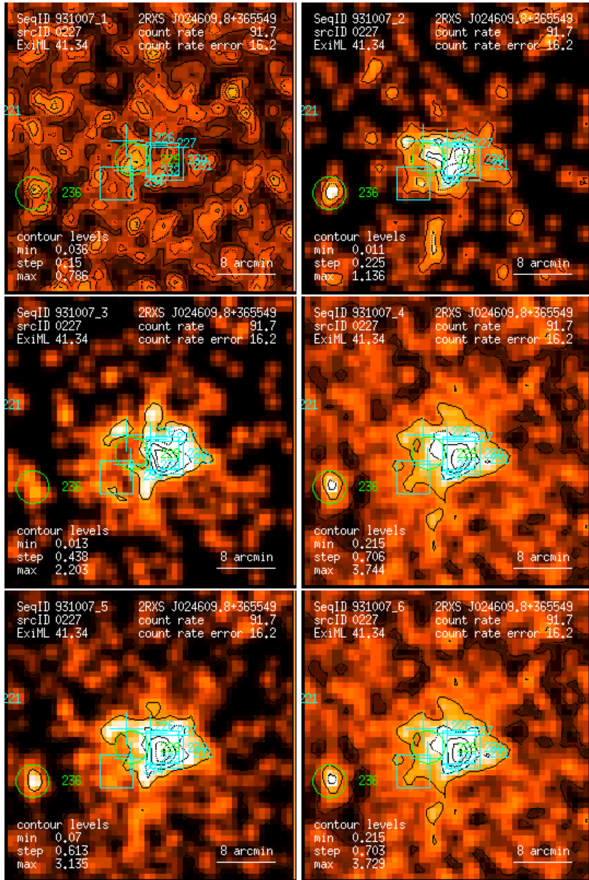
Figure 227: RASS 931007: detection 0227: band rate images, Gaussian filter: (1) PSPC channels 11 – 41, (2) 52 – 90, (3) 91 – 201, (4) 11 – 235, (5) 52 – 201, (6) 11 – 201. Broad band rates in counts/ks. Band rate contour levels in counts/ks/arcmin 2 .
