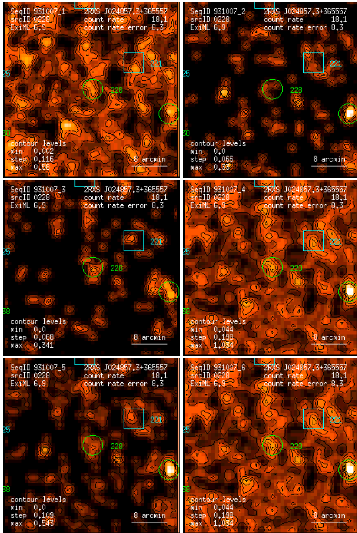
Figure 228: RASS 931007: detection 0228: band rate images, Gaussian filter: (1) PSPC channels 11 – 41, (2) 52 – 90, (3) 91 – 201, (4) 11 – 235, (5) 52 – 201, (6) 11 – 201. Broad band rates in counts/ks. Band rate contour levels in counts/ks/arcmin 2 .
