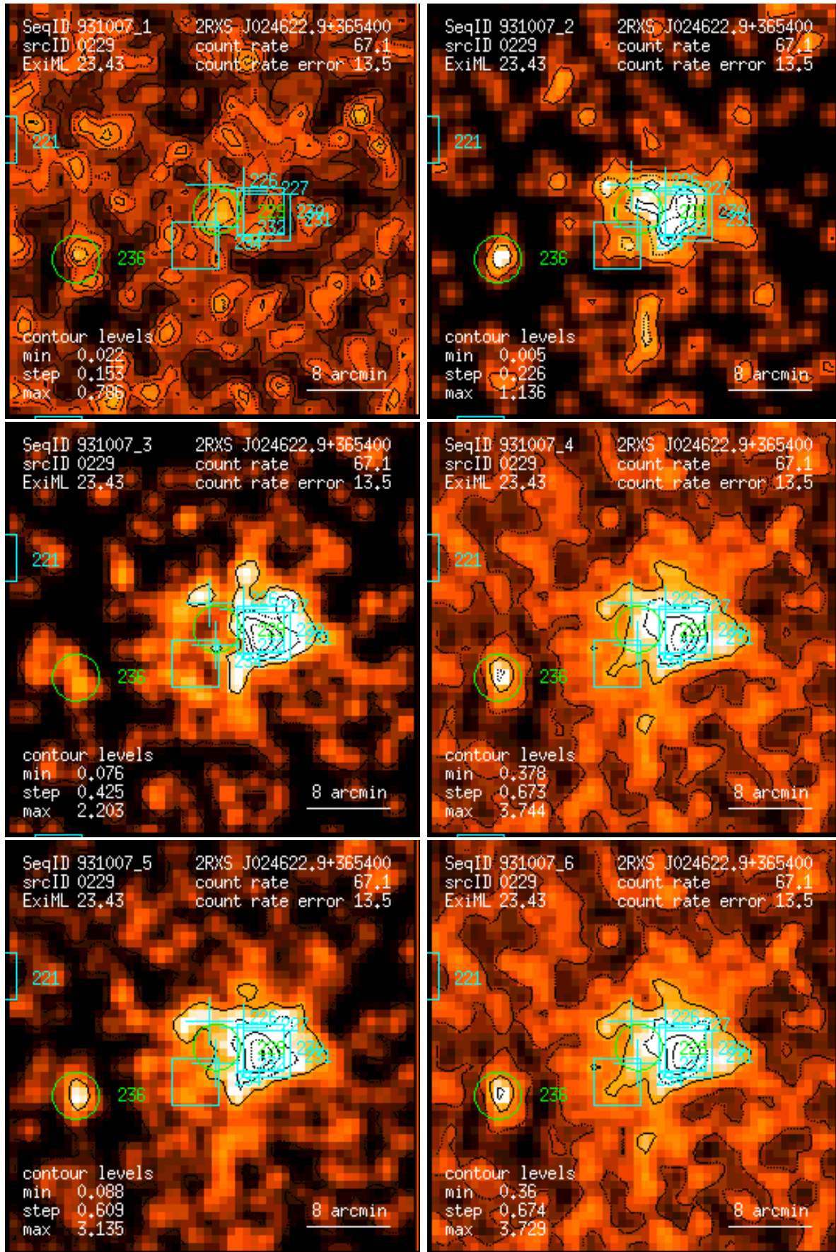
Figure 229: RASS 931007: detection 0229: band rate images, Gaussian filter: (1) PSPC channels 11 – 41, (2) 52 – 90, (3) 91 – 201, (4) 11 – 235, (5) 52 – 201, (6) 11 – 201. Broad band rates in counts/ks. Band rate contour levels in counts/ks/arcmin 2 .
