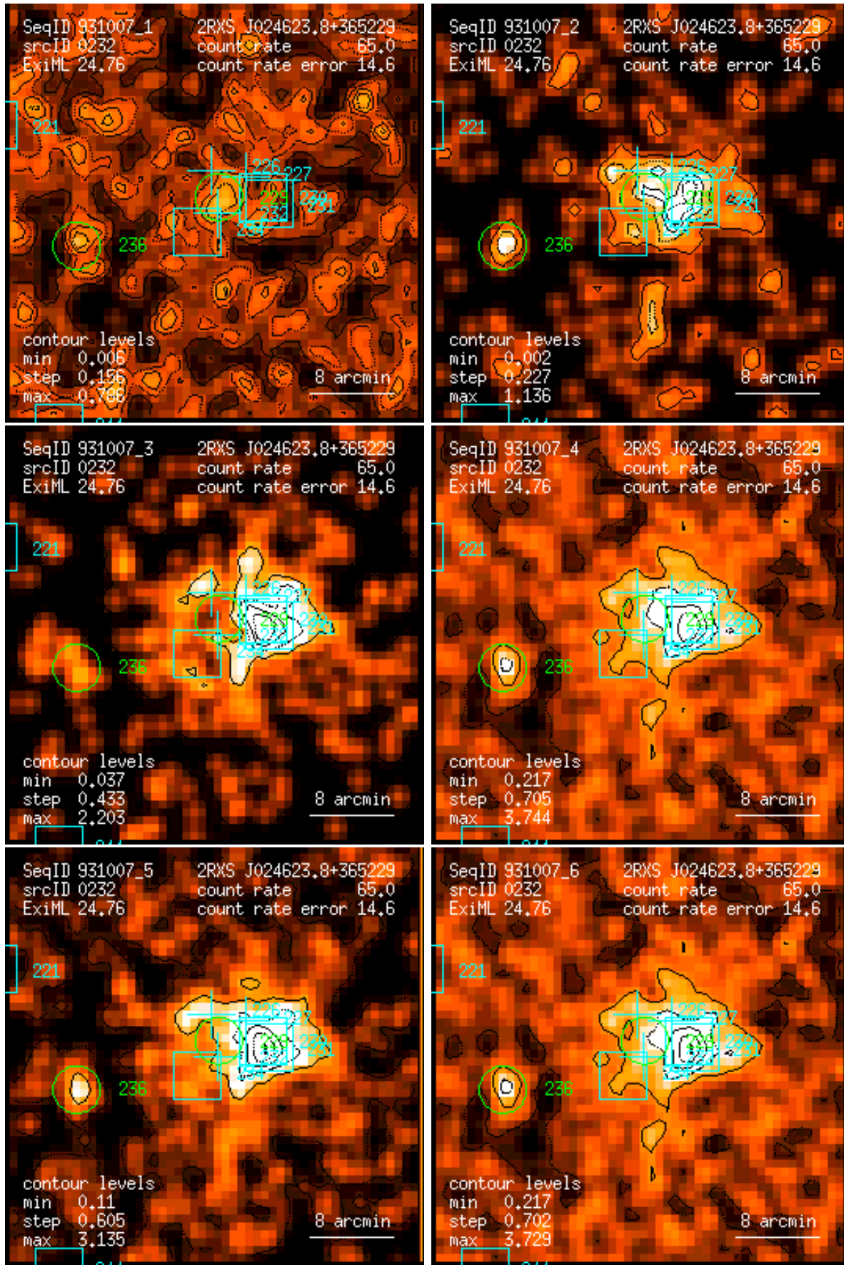
Figure 232: RASS 931007: detection 0232: band rate images, Gaussian filter: (1) PSPC channels 11 – 41, (2) 52 – 90, (3) 91 – 201, (4) 11 – 235, (5) 52 – 201, (6) 11 – 201. Broad band rates in counts/ks. Band rate contour levels in counts/ks/arcmin 2 .
