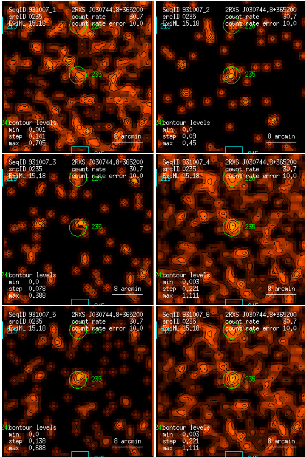
Figure 235: RASS 931007: detection 0235: band rate images, Gaussian filter: (1) PSPC channels 11 – 41, (2) 52 – 90, (3) 91 – 201, (4) 11 – 235, (5) 52 – 201, (6) 11 – 201. Broad band rates in counts/ks. Band rate contour levels in counts/ks/arcmin 2 .
