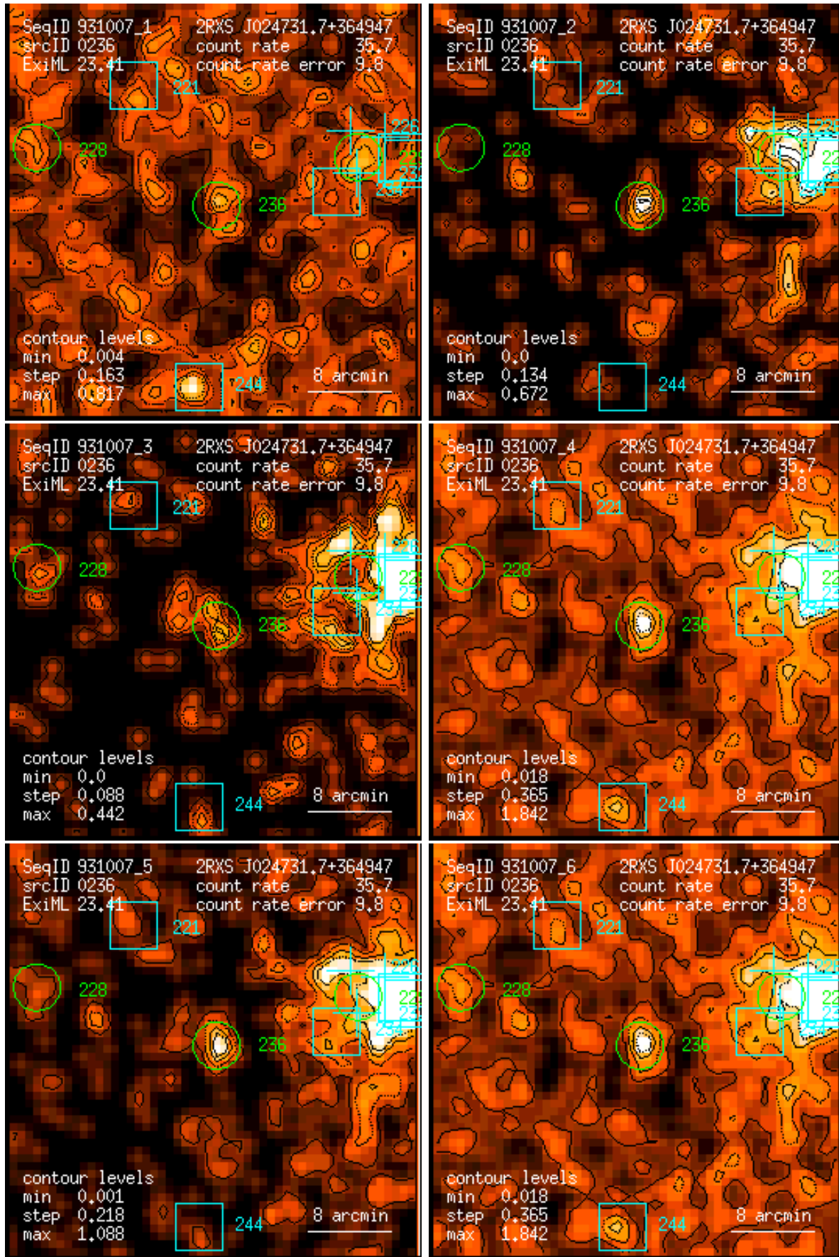
Figure 236: RASS 931007: detection 0236: band rate images, Gaussian filter: (1) PSPC channels 11 – 41, (2) 52 – 90, (3) 91 – 201, (4) 11 – 235, (5) 52 – 201, (6) 11 – 201. Broad band rates in counts/ks. Band rate contour levels in counts/ks/arcmin 2 .
