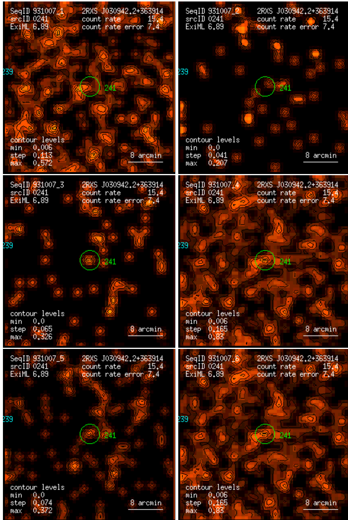
Figure 241: RASS 931007: detection 0241: band rate images, Gaussian filter: (1) PSPC channels 11 – 41, (2) 52 – 90, (3) 91 – 201, (4) 11 – 235, (5) 52 – 201, (6) 11 – 201. Broad band rates in counts/ks. Band rate contour levels in counts/ks/arcmin 2 .
