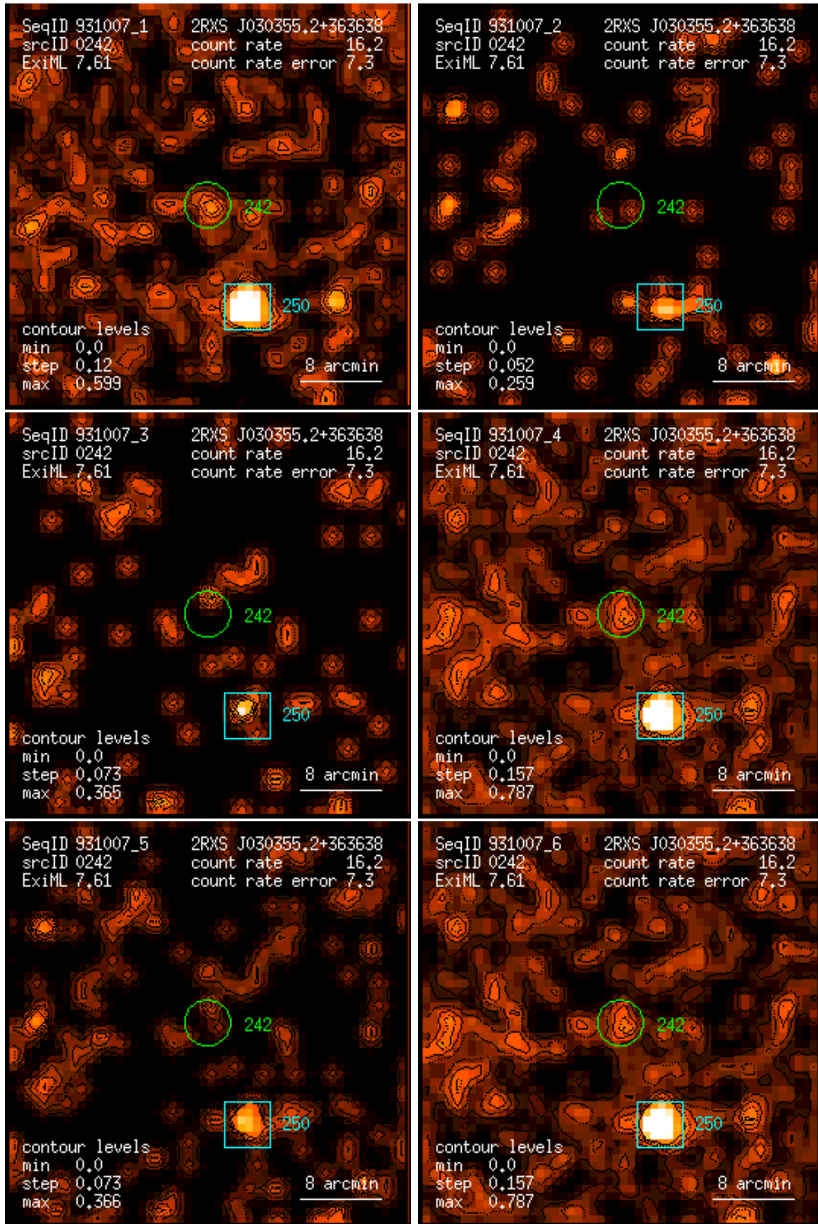
Figure 242: RASS 931007: detection 0242: band rate images, Gaussian filter: (1) PSPC channels 11 – 41, (2) 52 – 90, (3) 91 – 201, (4) 11 – 235, (5) 52 – 201, (6) 11 – 201. Broad band rates in counts/ks. Band rate contour levels in counts/ks/arcmin 2 .
