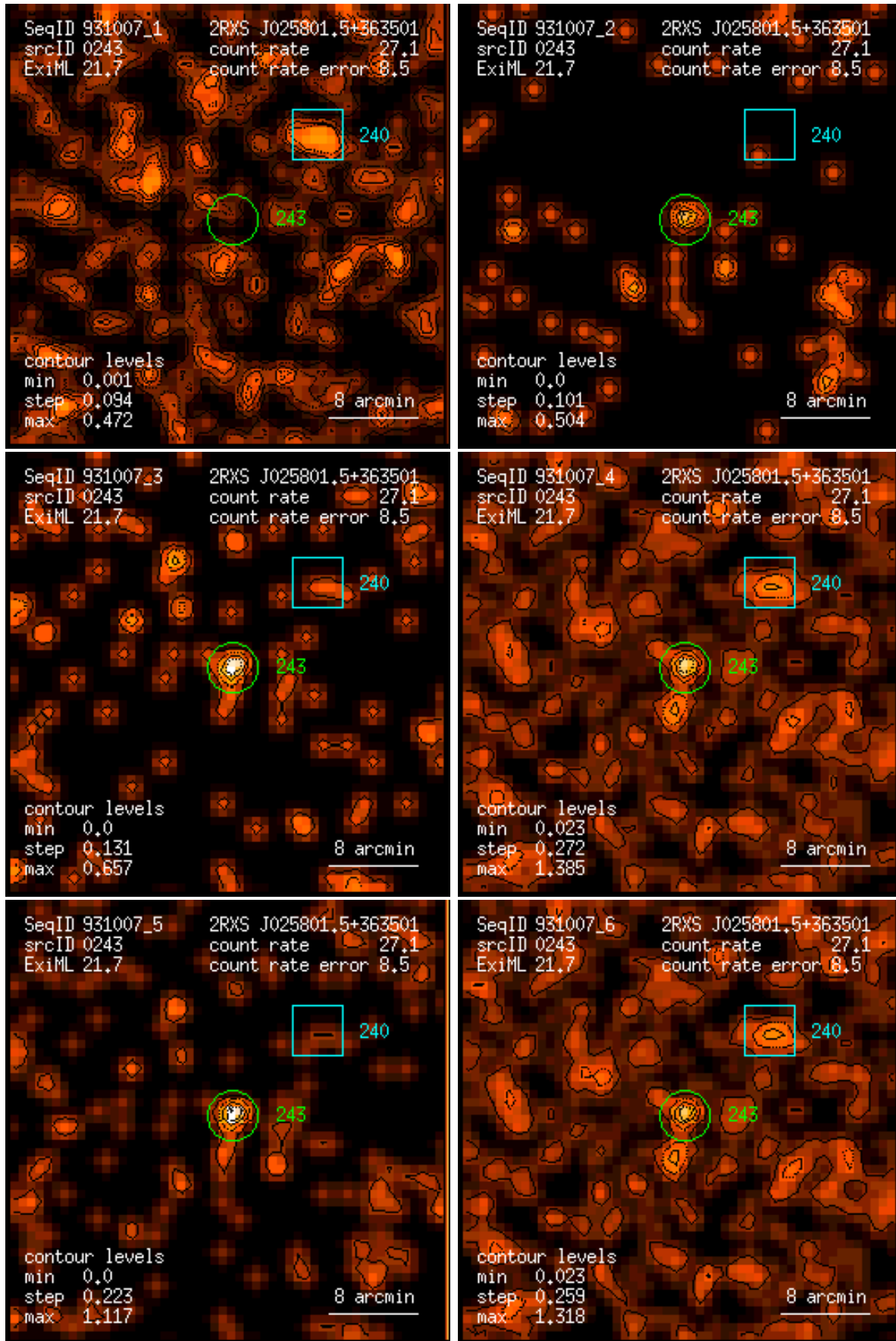
Figure 243: RASS 931007: detection 0243: band rate images, Gaussian filter: (1) PSPC channels 11 – 41, (2) 52 – 90, (3) 91 – 201, (4) 11 – 235, (5) 52 – 201, (6) 11 – 201. Broad band rates in counts/ks. Band rate contour levels in counts/ks/arcmin 2 .
