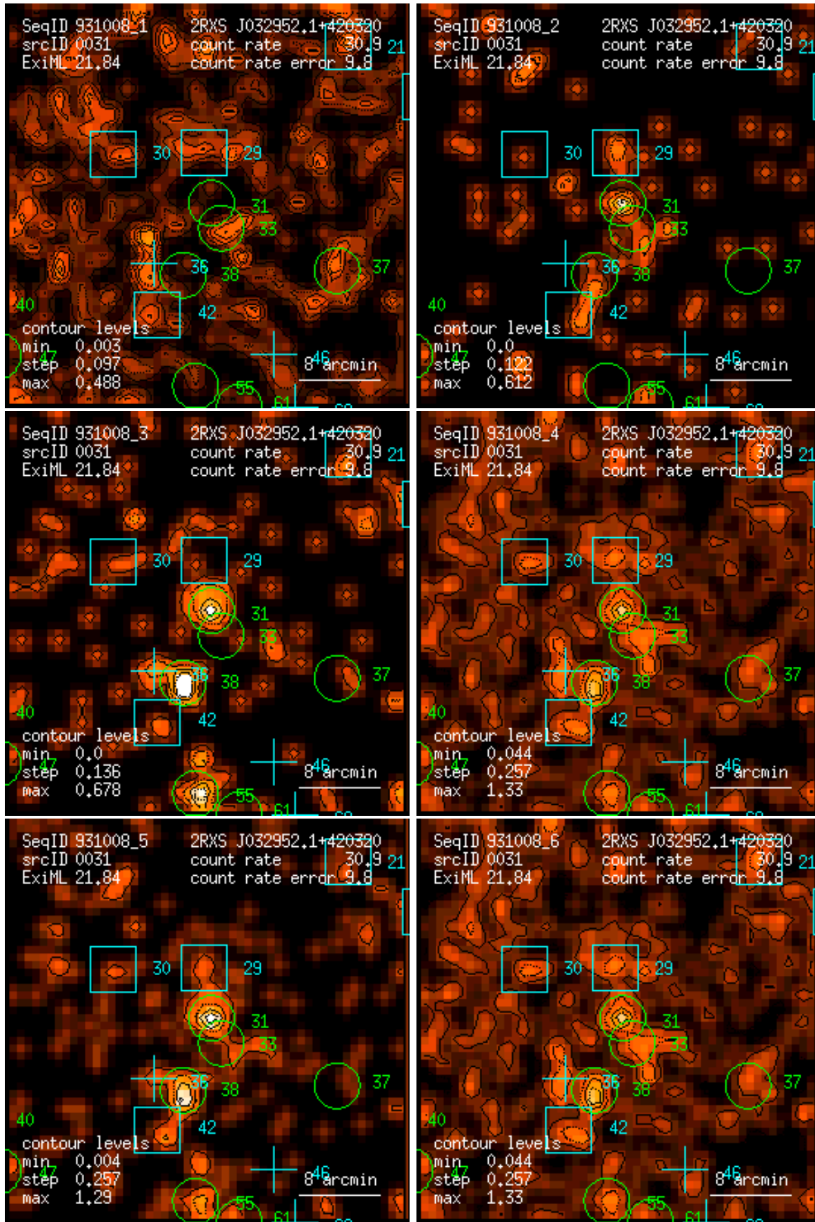
Figure 31: RASS 931008: detection 0031: band rate images, Gaussian filter: (1) PSPC channels 11 – 41, (2) 52 – 90, (3) 91 – 201, (4) 11 – 235, (5) 52 – 201, (6) 11 – 201. Broad band rates in counts/ks. Band rate contour levels in counts/ks/arcmin 2 .
