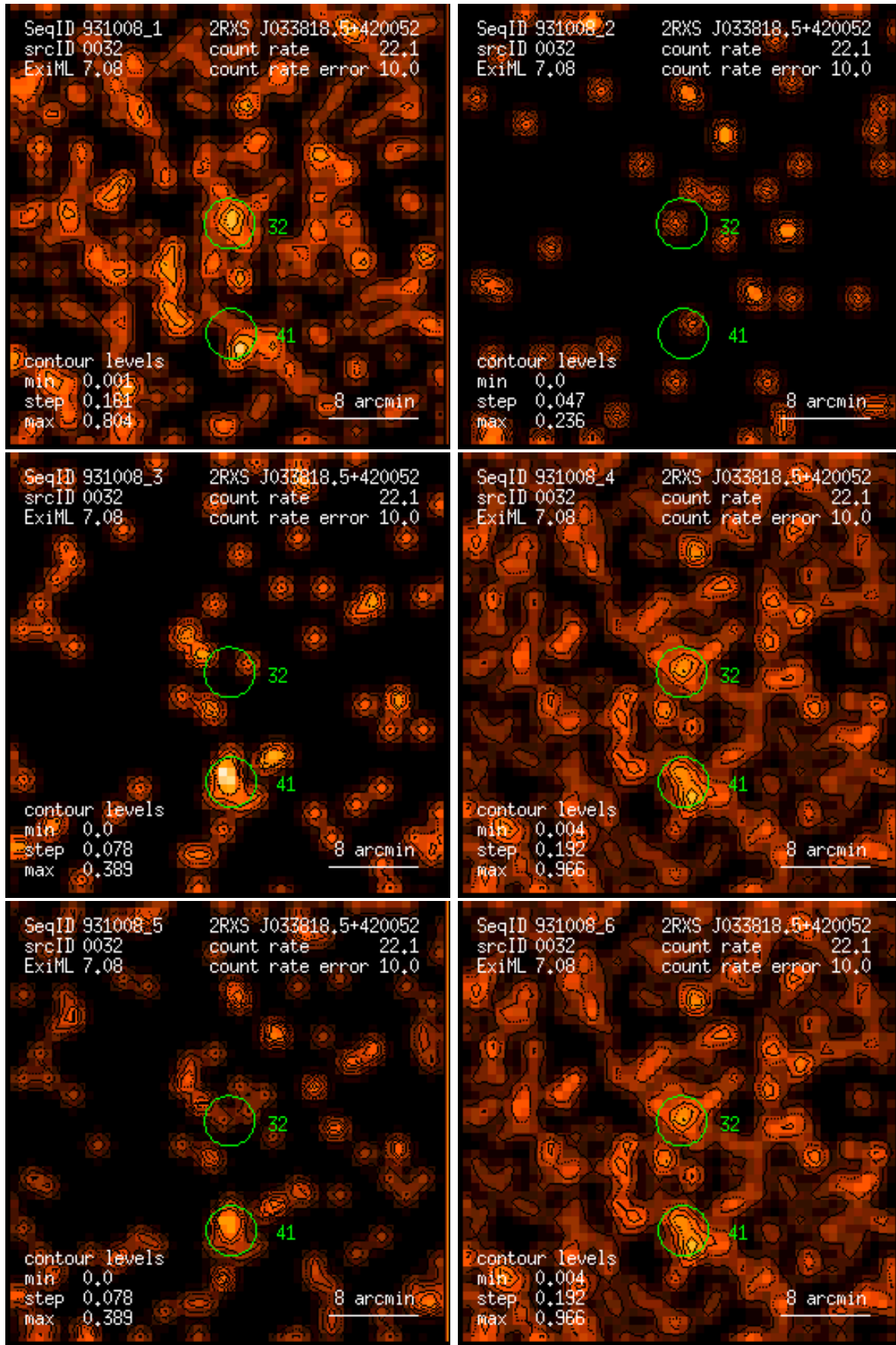
Figure 32: RASS 931008: detection 0032: band rate images, Gaussian filter: (1) PSPC channels 11 – 41, (2) 52 – 90, (3) 91 – 201, (4) 11 – 235, (5) 52 – 201, (6) 11 – 201. Broad band rates in counts/ks. Band rate contour levels in counts/ks/arcmin 2 .
