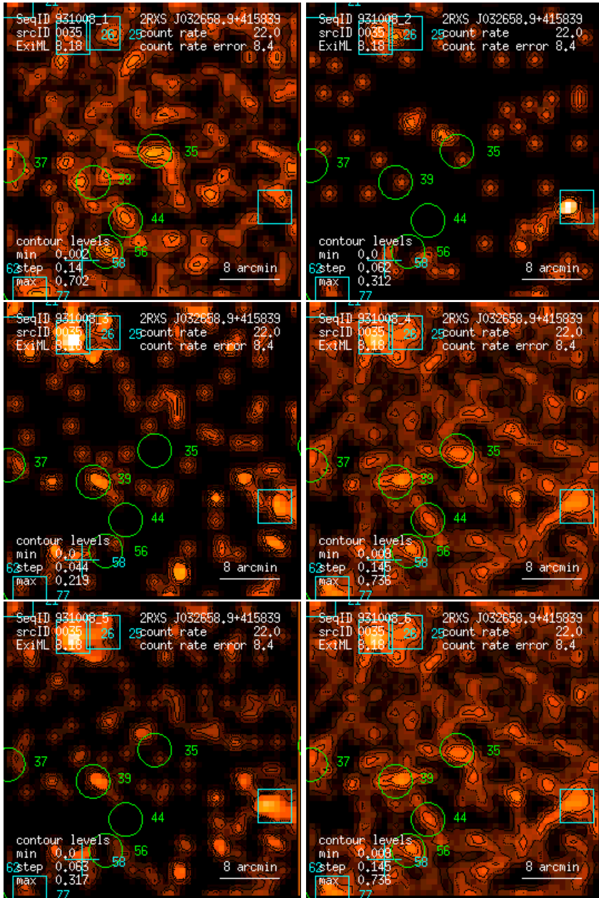
Figure 35: RASS 931008: detection 0035: band rate images, Gaussian filter: (1) PSPC channels 11 – 41, (2) 52 – 90, (3) 91 – 201, (4) 11 – 235, (5) 52 – 201, (6) 11 – 201. Broad band rates in counts/ks. Band rate contour levels in counts/ks/arcmin 2 .
