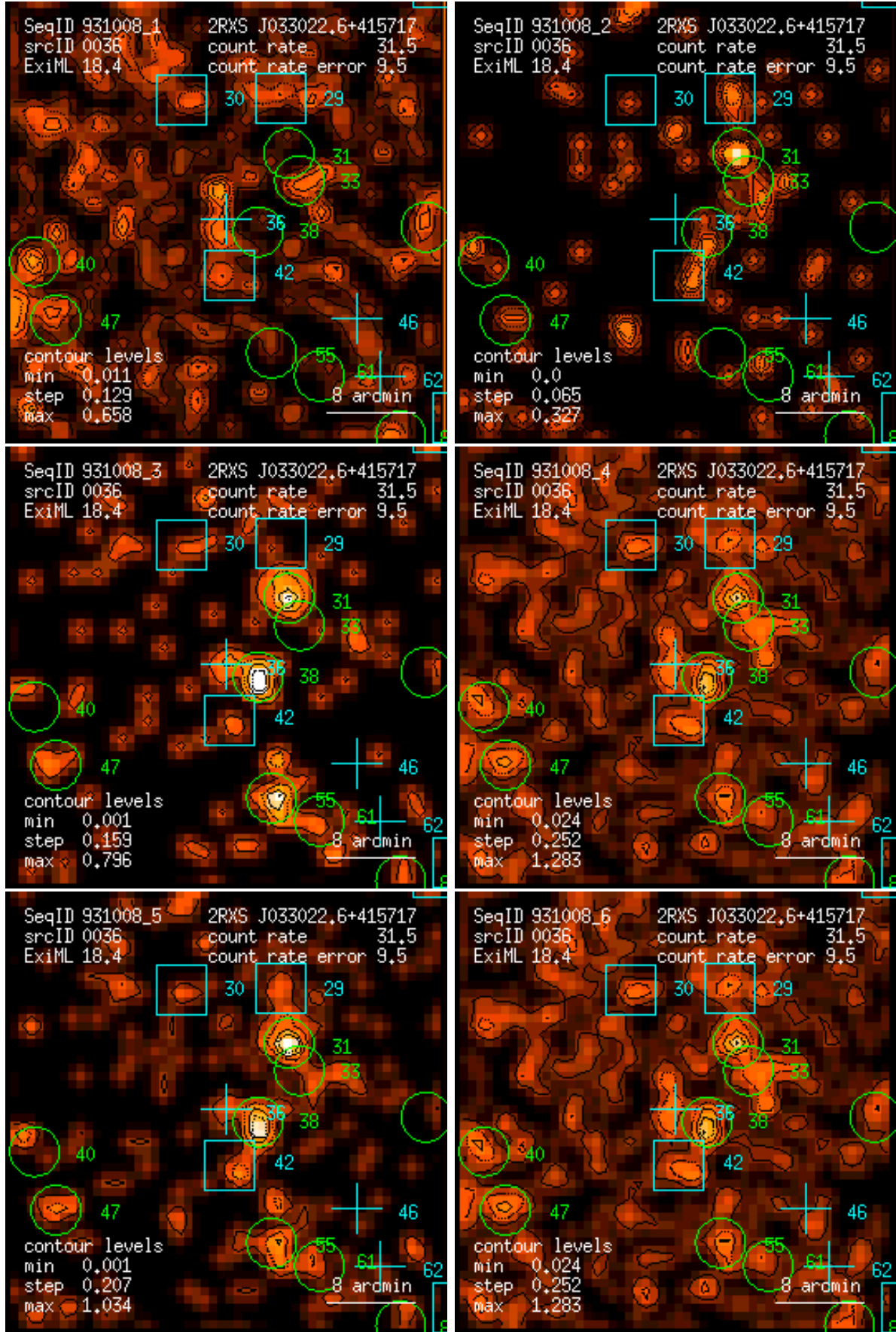
Figure 36: RASS 931008: detection 0036: band rate images, Gaussian filter: (1) PSPC channels 11 – 41, (2) 52 – 90, (3) 91 – 201, (4) 11 – 235, (5) 52 – 201, (6) 11 – 201. Broad band rates in counts/ks. Band rate contour levels in counts/ks/arcmin 2 .
