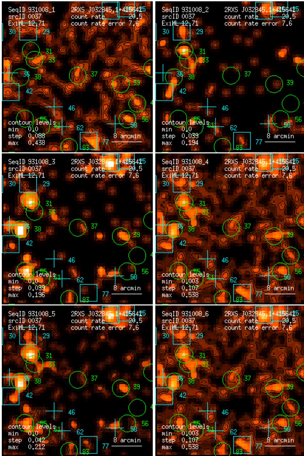
Figure 37: RASS 931008: detection 0037: band rate images, Gaussian filter: (1) PSPC channels 11 – 41, (2) 52 – 90, (3) 91 – 201, (4) 11 – 235, (5) 52 – 201, (6) 11 – 201. Broad band rates in counts/ks. Band rate contour levels in counts/ks/arcmin 2 .
