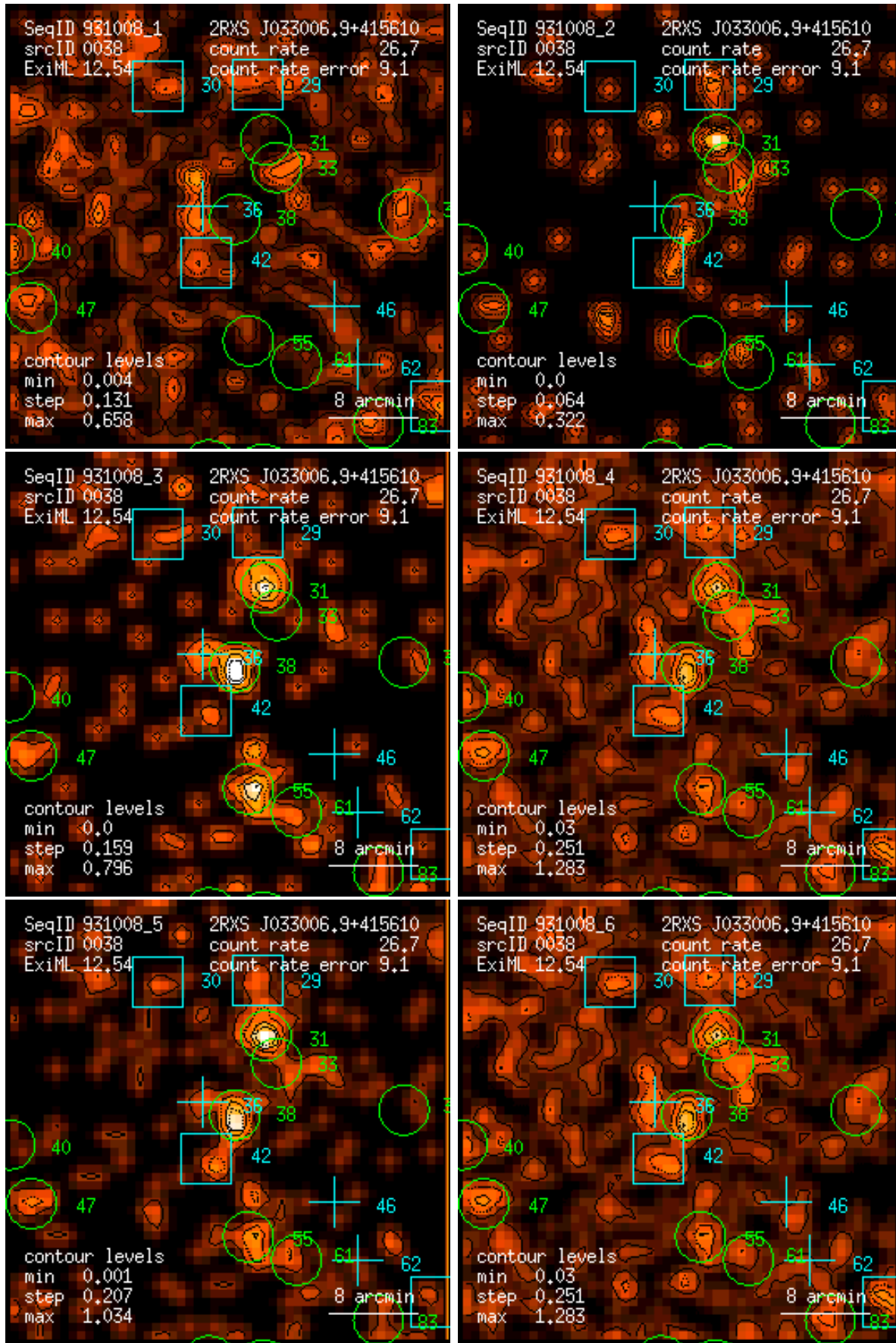
Figure 38: RASS 931008: detection 0038: band rate images, Gaussian filter: (1) PSPC channels 11 – 41, (2) 52 – 90, (3) 91 – 201, (4) 11 – 235, (5) 52 – 201, (6) 11 – 201. Broad band rates in counts/ks. Band rate contour levels in counts/ks/arcmin 2 .
