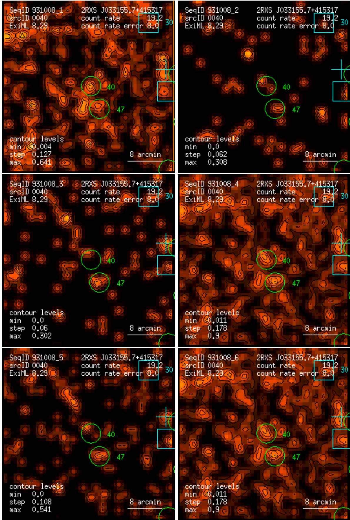
Figure 40: RASS 931008: detection 0040: band rate images, Gaussian filter: (1) PSPC channels 11 – 41, (2) 52 – 90, (3) 91 – 201, (4) 11 – 235, (5) 52 – 201, (6) 11 – 201. Broad band rates in counts/ks. Band rate contour levels in counts/ks/arcmin 2 .
