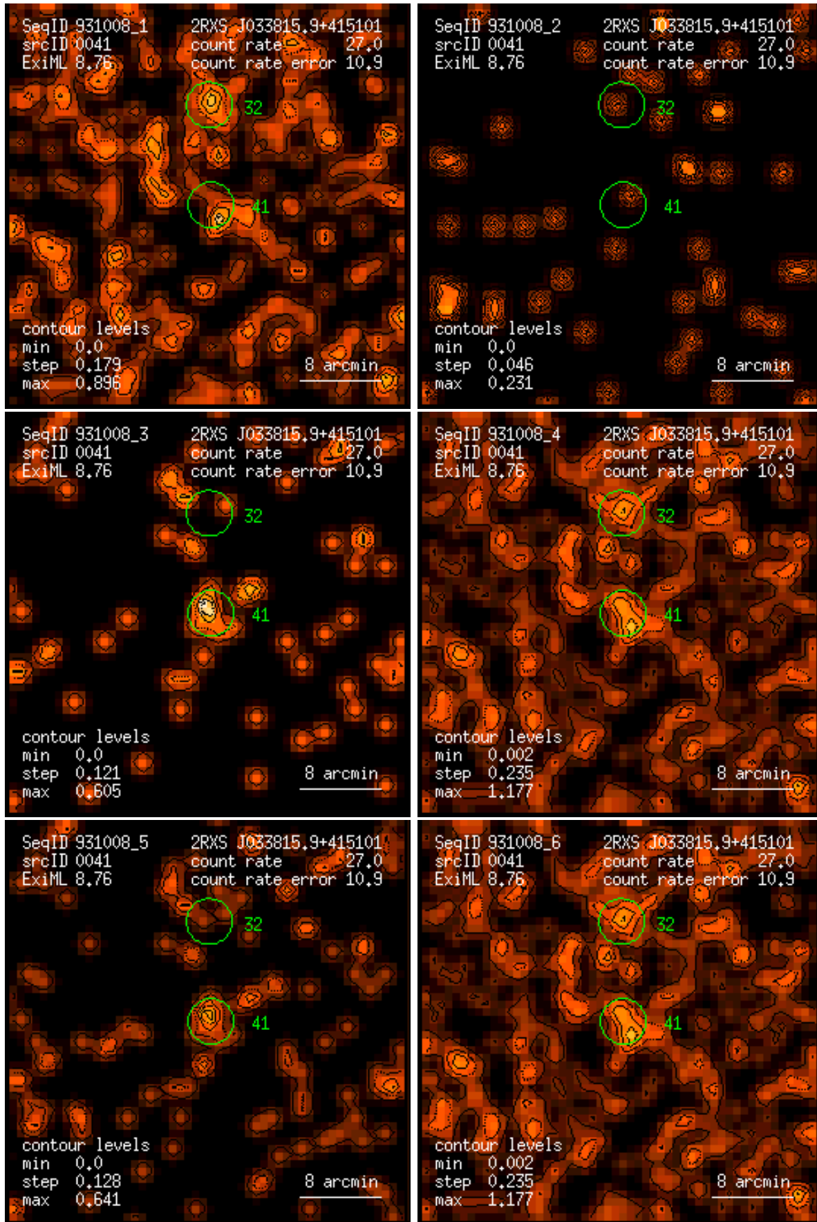
Figure 41: RASS 931008: detection 0041: band rate images, Gaussian filter: (1) PSPC channels 11 – 41, (2) 52 – 90, (3) 91 – 201, (4) 11 – 235, (5) 52 – 201, (6) 11 – 201. Broad band rates in counts/ks. Band rate contour levels in counts/ks/arcmin 2 .
