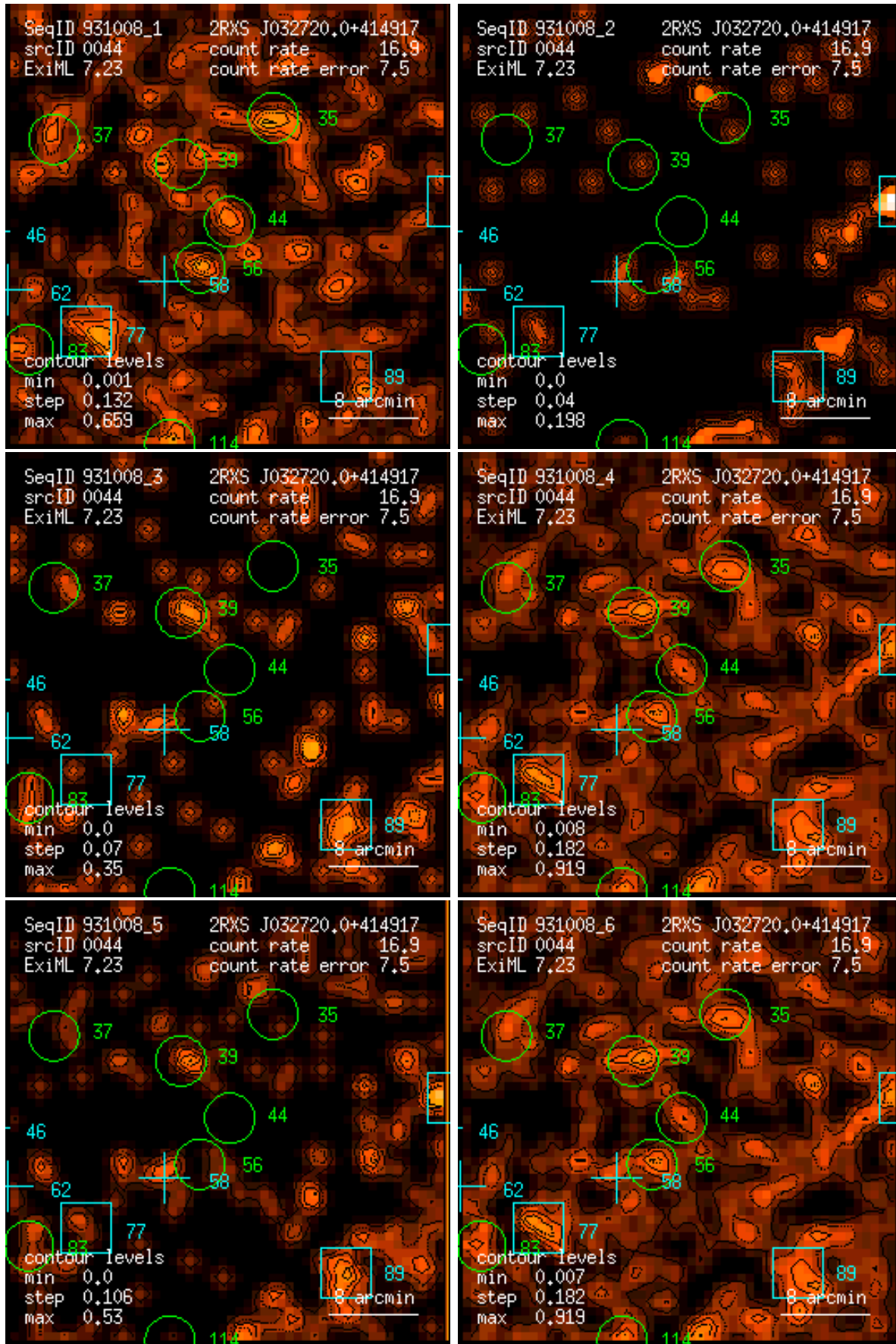
Figure 44: RASS 931008: detection 0044: band rate images, Gaussian filter: (1) PSPC channels 11 – 41, (2) 52 – 90, (3) 91 – 201, (4) 11 – 235, (5) 52 – 201, (6) 11 – 201. Broad band rates in counts/ks. Band rate contour levels in counts/ks/arcmin 2 .
