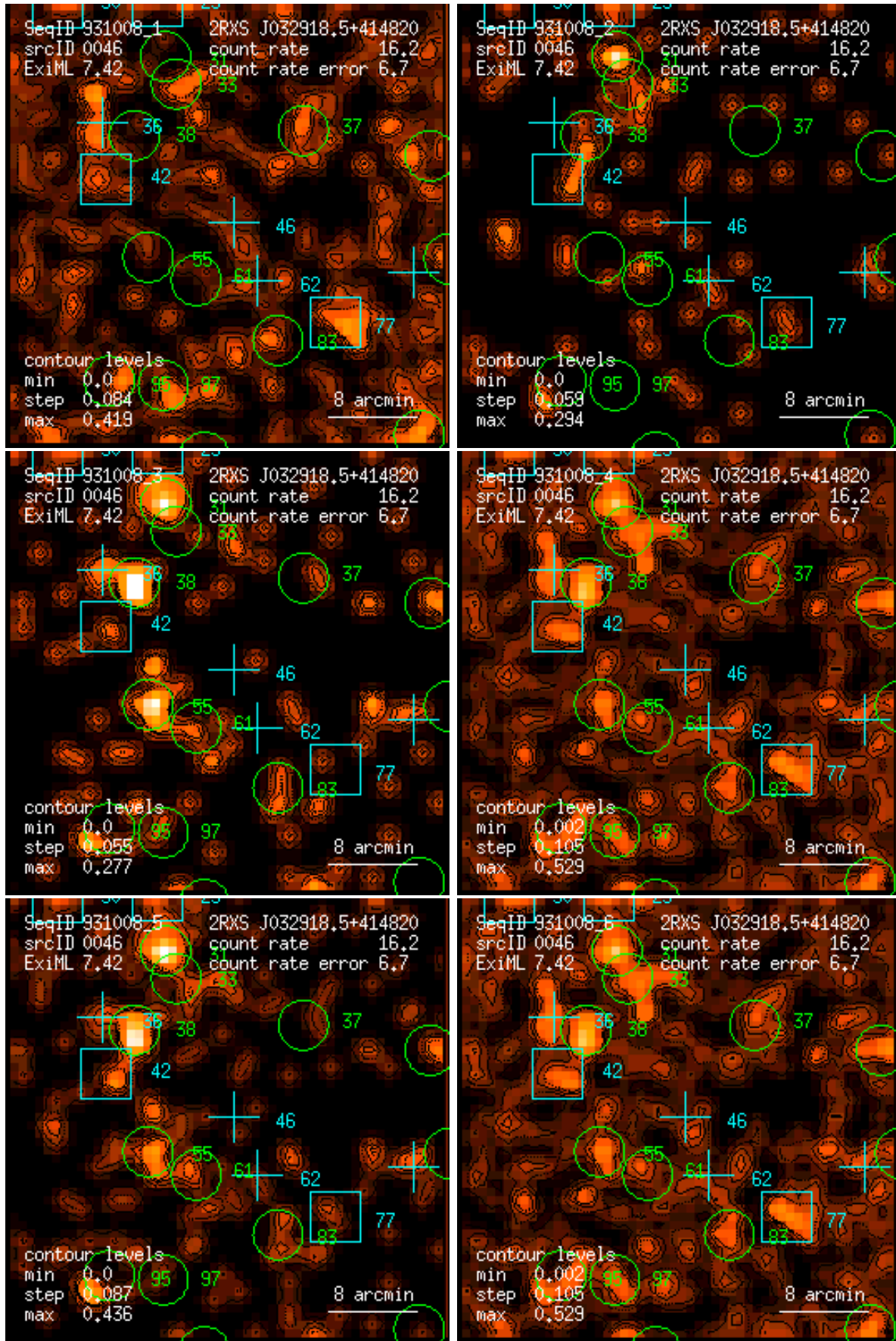
Figure 46: RASS 931008: detection 0046: band rate images, Gaussian filter: (1) PSPC channels 11 – 41, (2) 52 – 90, (3) 91 – 201, (4) 11 – 235, (5) 52 – 201, (6) 11 – 201. Broad band rates in counts/ks. Band rate contour levels in counts/ks/arcmin 2 .
