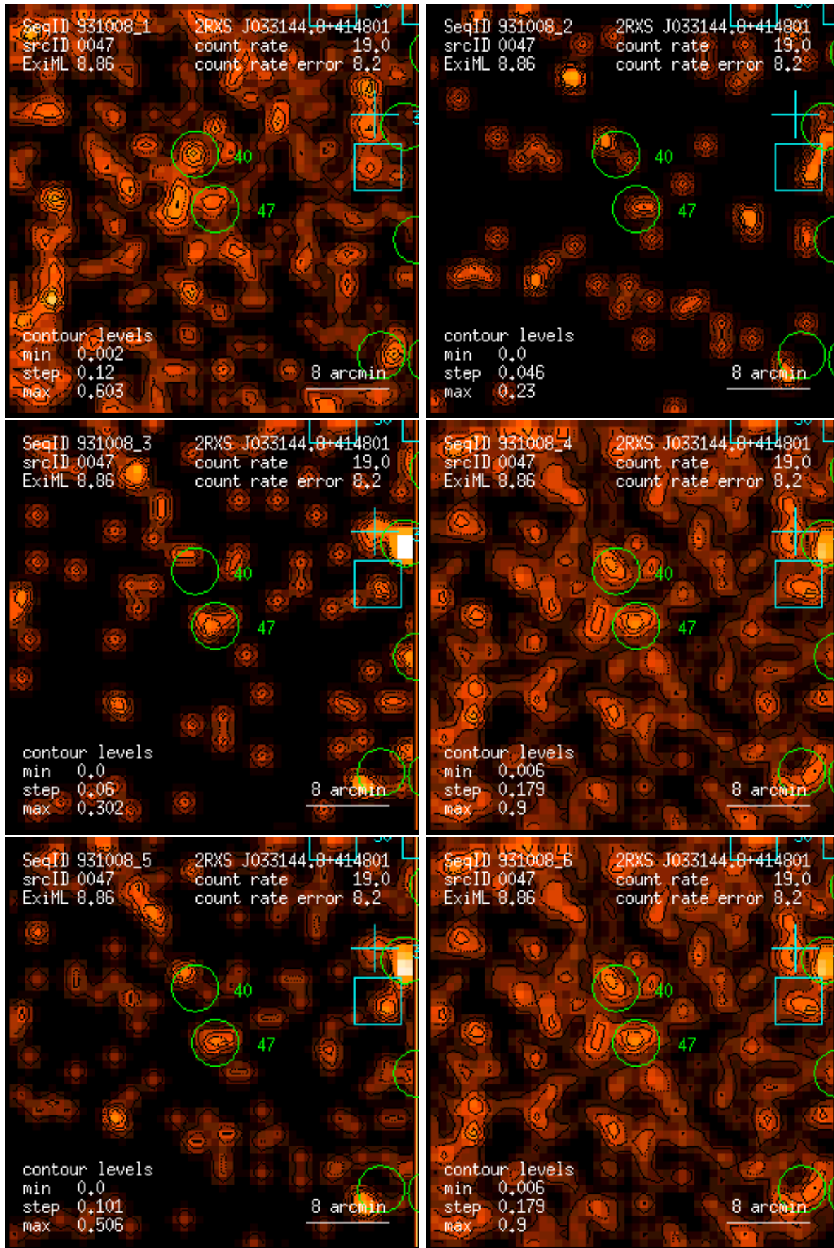
Figure 47: RASS 931008: detection 0047: band rate images, Gaussian filter: (1) PSPC channels 11 – 41, (2) 52 – 90, (3) 91 – 201, (4) 11 – 235, (5) 52 – 201, (6) 11 – 201. Broad band rates in counts/ks. Band rate contour levels in counts/ks/arcmin 2 .
