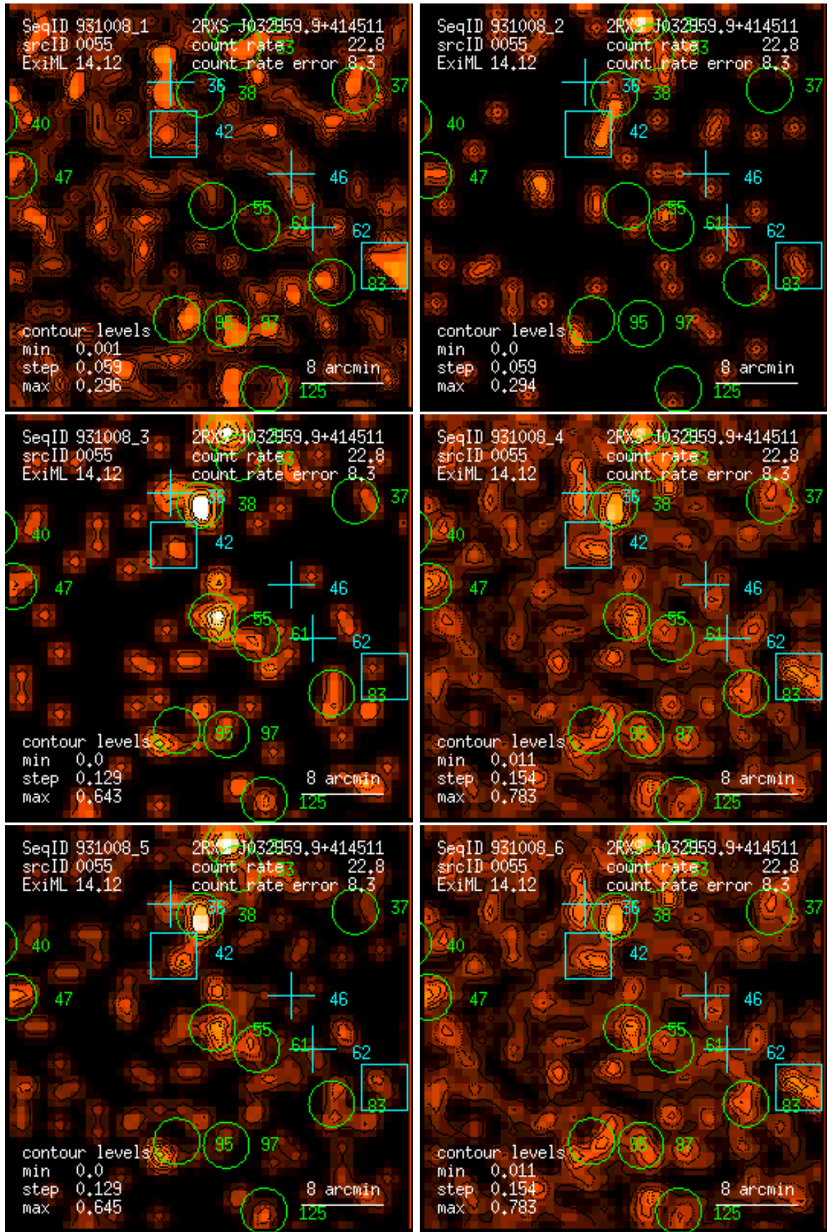
Figure 55: RASS 931008: detection 0055: band rate images, Gaussian filter: (1) PSPC channels 11 – 41, (2) 52 – 90, (3) 91 – 201, (4) 11 – 235, (5) 52 – 201, (6) 11 – 201. Broad band rates in counts/ks. Band rate contour levels in counts/ks/arcmin 2 .
