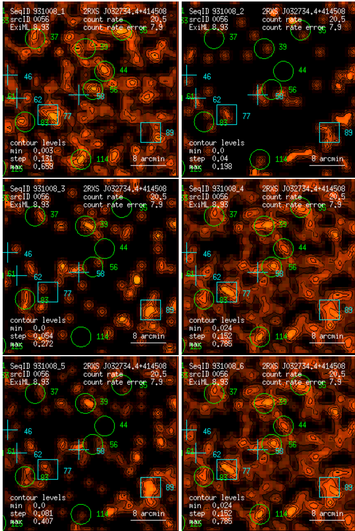
Figure 56: RASS 931008: detection 0056: band rate images, Gaussian filter: (1) PSPC channels 11 – 41, (2) 52 – 90, (3) 91 – 201, (4) 11 – 235, (5) 52 – 201, (6) 11 – 201. Broad band rates in counts/ks. Band rate contour levels in counts/ks/arcmin 2 .
