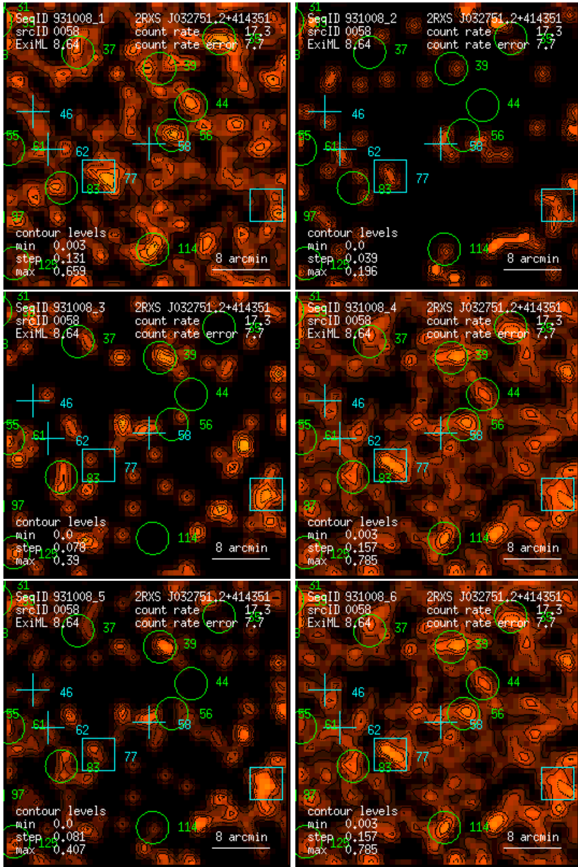
Figure 58: RASS 931008: detection 0058: band rate images, Gaussian filter: (1) PSPC channels 11 – 41, (2) 52 – 90, (3) 91 – 201, (4) 11 – 235, (5) 52 – 201, (6) 11 – 201. Broad band rates in counts/ks. Band rate contour levels in counts/ks/arcmin 2 .
