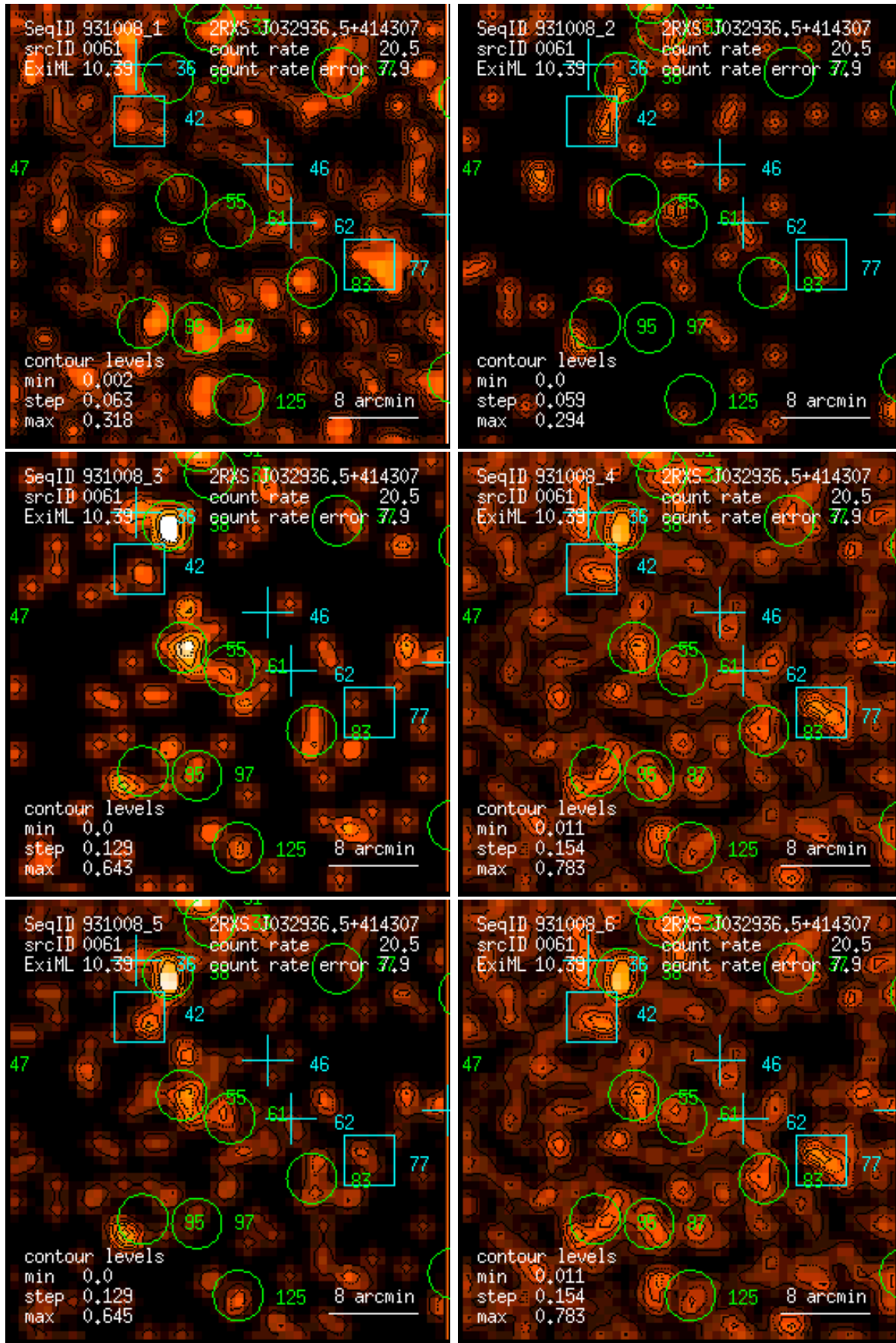
Figure 61: RASS 931008: detection 0061: band rate images, Gaussian filter: (1) PSPC channels 11 – 41, (2) 52 – 90, (3) 91 – 201, (4) 11 – 235, (5) 52 – 201, (6) 11 – 201. Broad band rates in counts/ks. Band rate contour levels in counts/ks/arcmin 2 .
