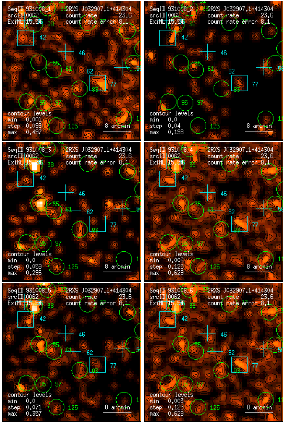
Figure 62: RASS 931008: detection 0062: band rate images, Gaussian filter: (1) PSPC channels 11 – 41, (2) 52 – 90, (3) 91 – 201, (4) 11 – 235, (5) 52 – 201, (6) 11 – 201. Broad band rates in counts/ks. Band rate contour levels in counts/ks/arcmin 2 .
