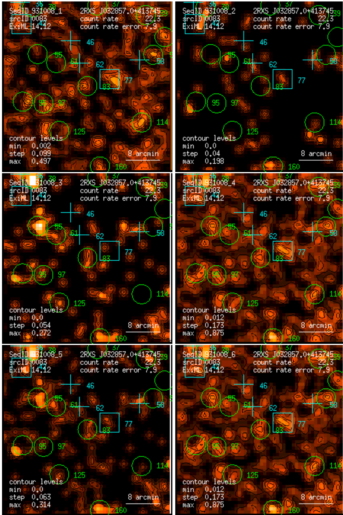
Figure 83: RASS 931008: detection 0083: band rate images, Gaussian filter: (1) PSPC channels 11 – 41, (2) 52 – 90, (3) 91 – 201, (4) 11 – 235, (5) 52 – 201, (6) 11 – 201. Broad band rates in counts/ks. Band rate contour levels in counts/ks/arcmin 2 .
