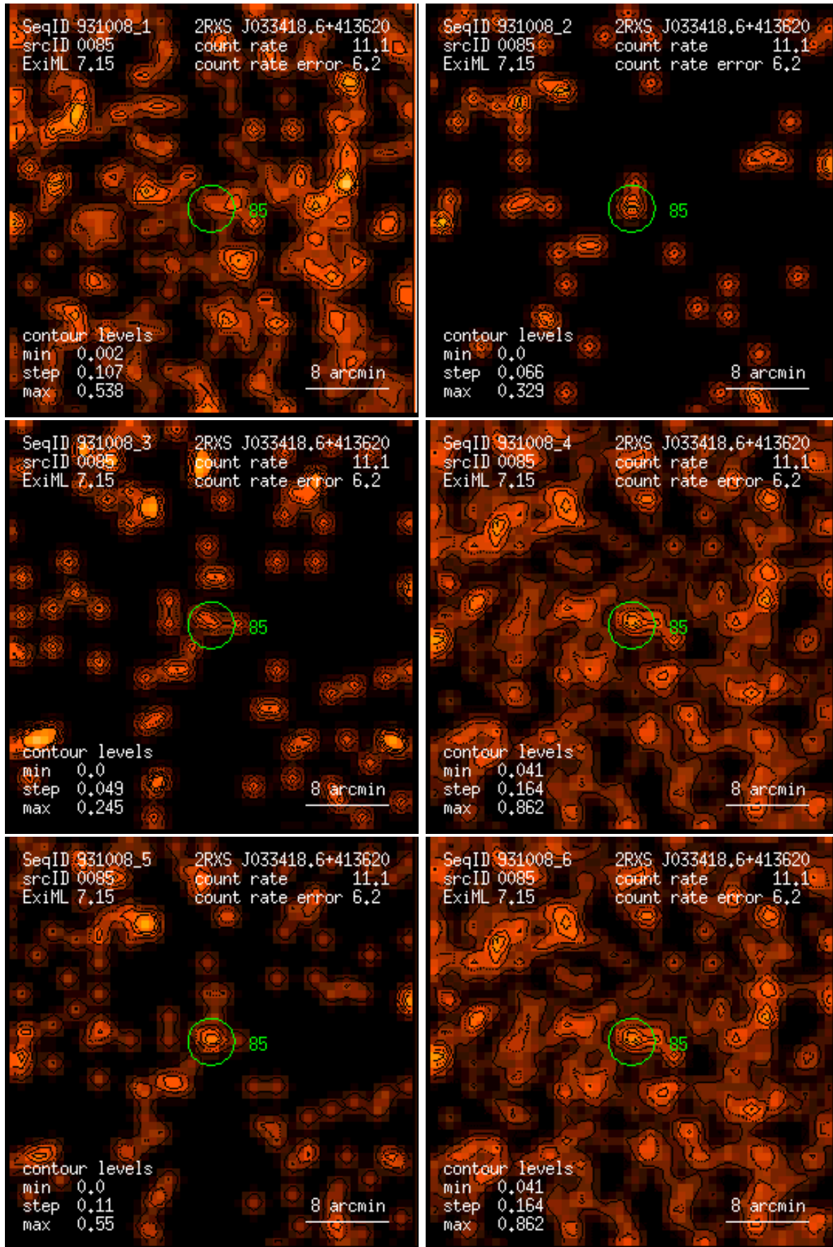
Figure 85: RASS 931008: detection 0085: band rate images, Gaussian filter: (1) PSPC channels 11 – 41, (2) 52 – 90, (3) 91 – 201, (4) 11 – 235, (5) 52 – 201, (6) 11 – 201. Broad band rates in counts/ks. Band rate contour levels in counts/ks/arcmin 2 .
