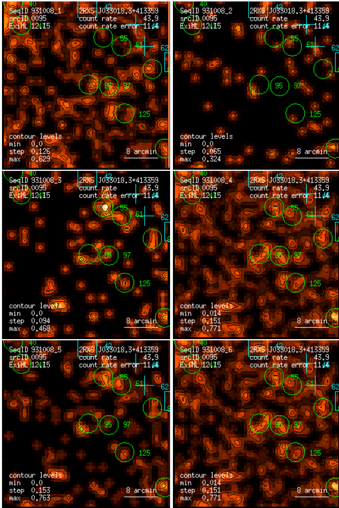
Figure 95: RASS 931008: detection 0095: band rate images, Gaussian filter: (1) PSPC channels 11 – 41, (2) 52 – 90, (3) 91 – 201, (4) 11 – 235, (5) 52 – 201, (6) 11 – 201. Broad band rates in counts/ks. Band rate contour levels in counts/ks/arcmin 2 .
